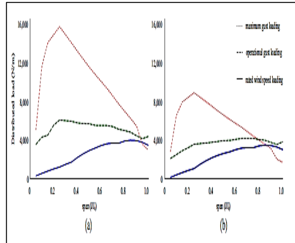
Figure (5): Comparison of aerodynamic loads on turbine blades at (a) high and (b) low wind speeds [36]
