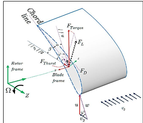
Figure (2): Distribution of aerodynamic forces acting on a wind turbine blade cross-section [28]
