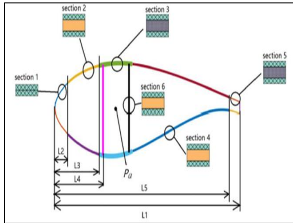
Figure (4): Typical structural configuration and parameters of a wind turbine blade section[32]
