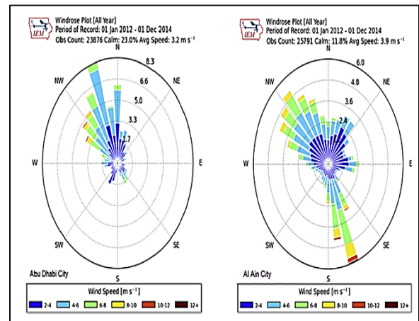
Figure (3): Wind rose diagrams for Abu Dhabi and Al Ain, illustrating prevailing wind directions and frequencies [31]
