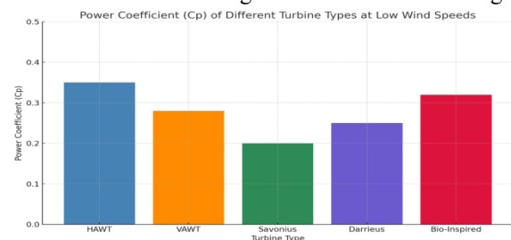
Figure (8): Power Coefficient (Cp) of Different Turbine Types at Low Wind Speeds Suggested [61]
