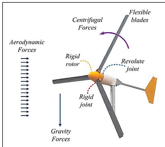
Figure (1): Schematic of a small-sized wind turbine modeled as a multi-body dynamic [28]
