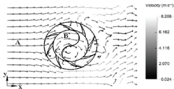
Figure (7): CFD simulation of wind flow through the wind booster[66]
