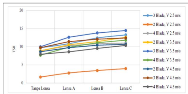
Figure (6): Impact of nozzle lens design on the power generation at various tip-speed ratios (TSR) [55]
