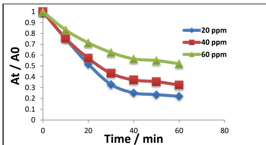
Fig. 3: Effect of dye concentration on the photocatalytic degradation at a constant weight of \text{Al}_2\text{O}_3
