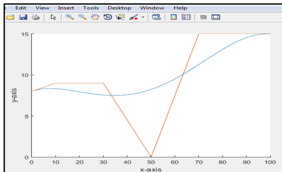
Figure 2. Bezier curves using MATLAB.
