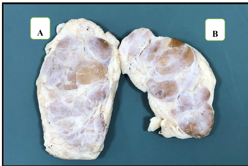
Fig.5 A: Left lobe and B : right lobe , Anatomical Structure of the Poll Gland in the Camel ( Camelus dromedarius ) During the non_ Breeding Season.
