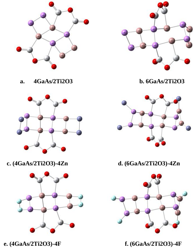
Fig.1: The molecular structure of the nanoclusters 4\text{GaAs}/2\text{Ti}_2\text{O}_3 , 6\text{GaAs}/2\text{Ti}_2\text{O}_3 , (4\text{GaAs}/2\text{Ti}_2\text{O}_3)-4\text{Zn} , (4\text{GaAs}/2\text{Ti}_2\text{O}_3)-4\text{F} , (6\text{GaAs}/2\text{Ti}_2\text{O}_3)-4\text{Zn} and (6\text{GaAs}/2\text{Ti}_2\text{O}_3)-4\text{F} .
