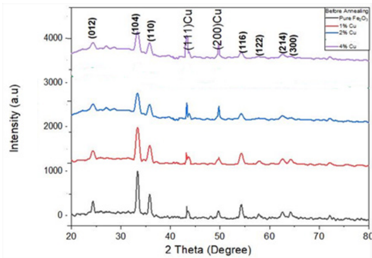
Figure (3) X-ray diffraction of iron oxide films.
