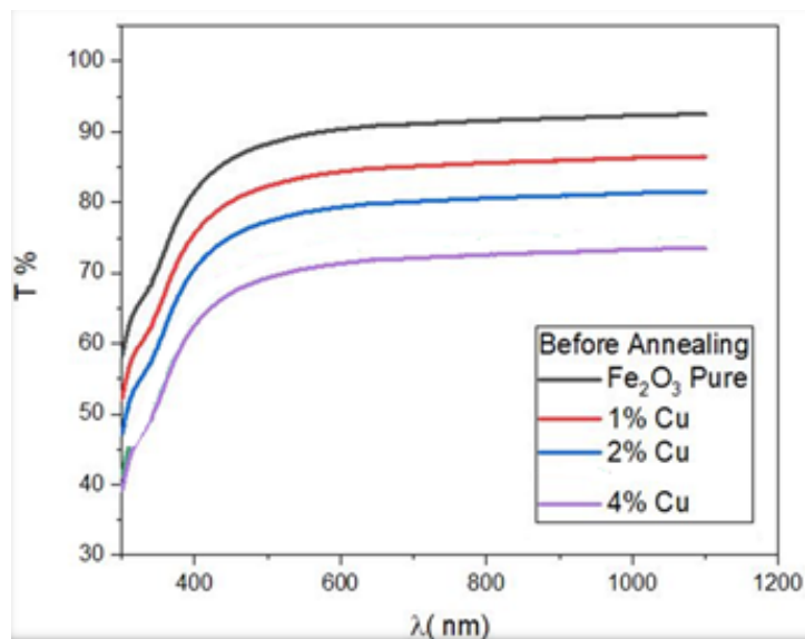
Figure (7) Transmittance spectrum of iron oxide films
