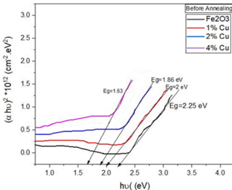
Figure (8) Energy gap of iron oxide films.
