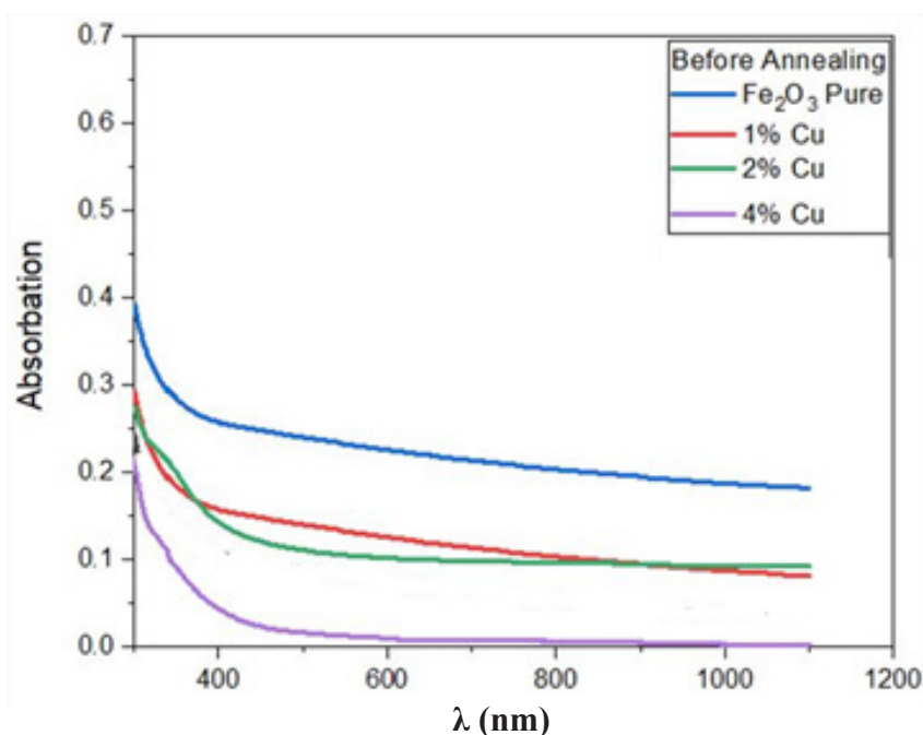
Figure (6) shows the absorption spectrum of iron oxide films:
