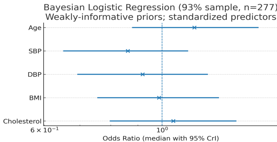
Figure 3. Posterior odds ratios (median with 95% credible intervals) from the Bayesian logistic regression on the large subset (93%, n=277) with weakly-informative Normal (0,1) priors and standardized predictors. A vertical dashed line at OR = 1 indicates no effect. WAIC = 327 and LOOIC = 327 ( \approx 1.18 per observation)
