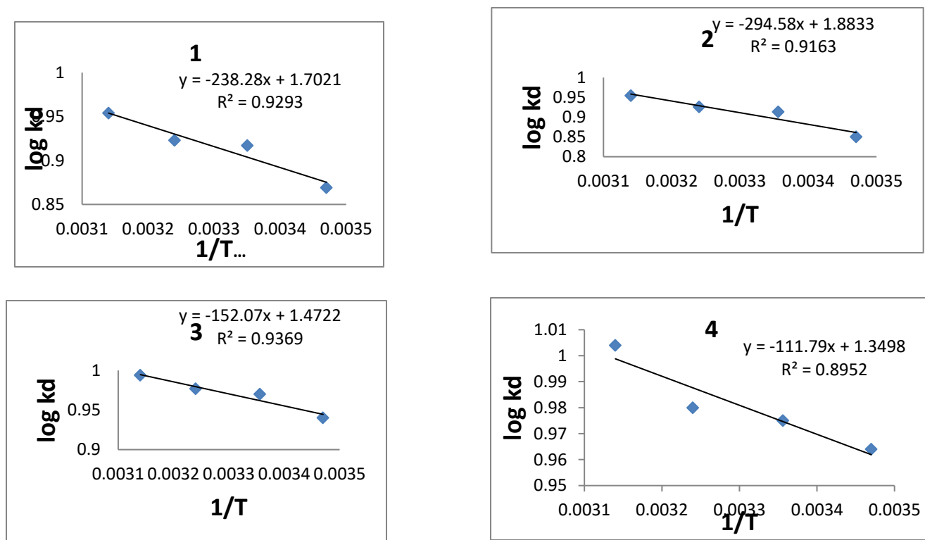
Figure 1: Linear relationship between Log Kd and 1/T for selenium adsorption on the study soil
