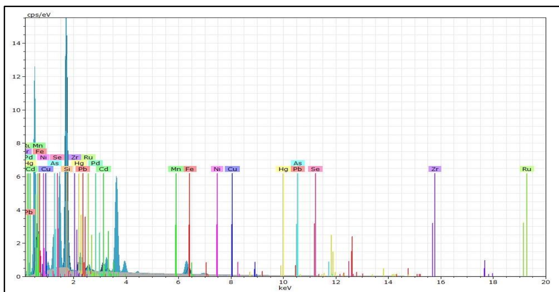
Fig. (3) EDX analysis of sample 1.
