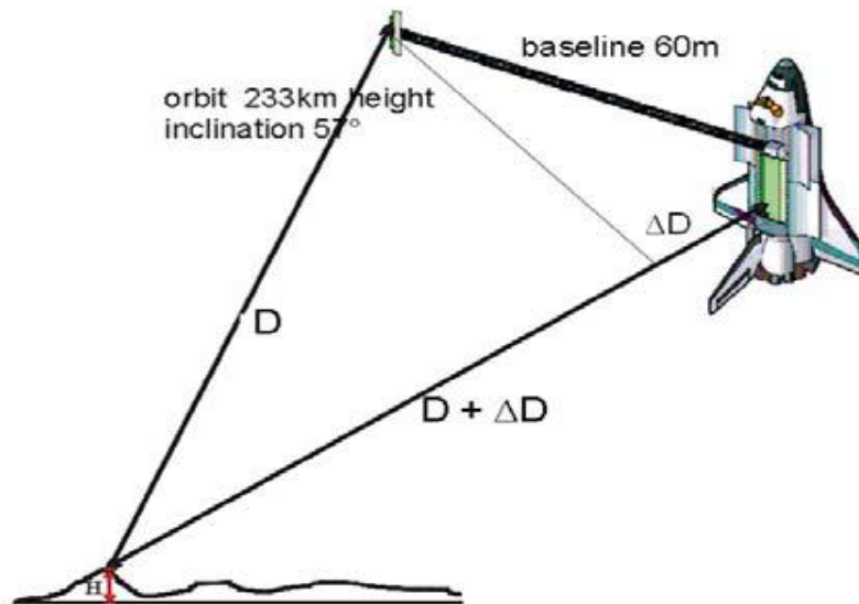
Figure (2) In SAR configuration.
