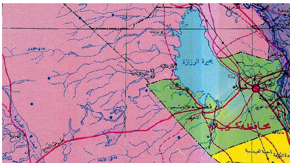
Figure (4) The study area lies west of Al Razzaza Lake.
