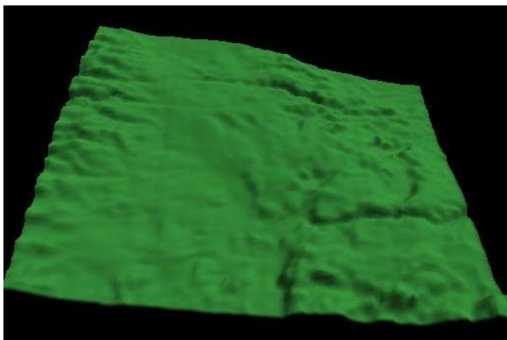
Figure (6) 3D view of the region.
