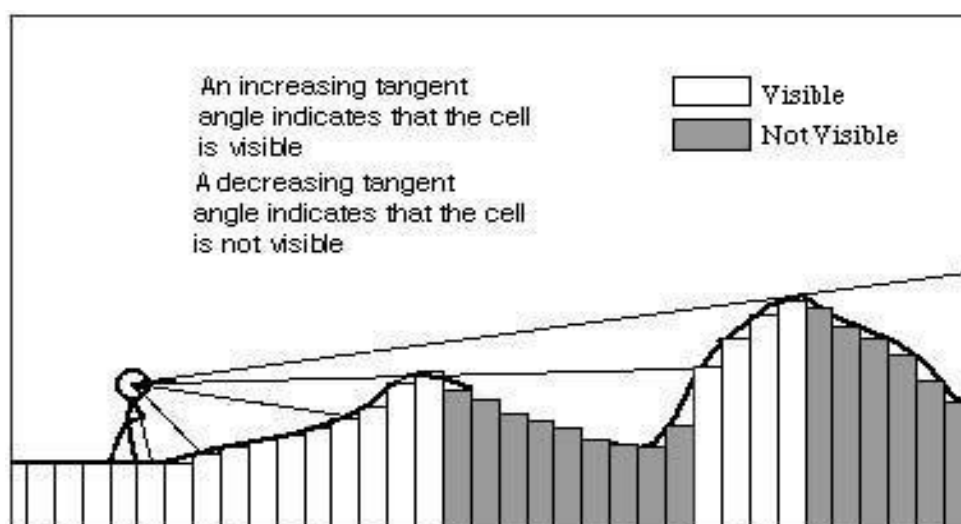
Figure (3) Line of Sight.
