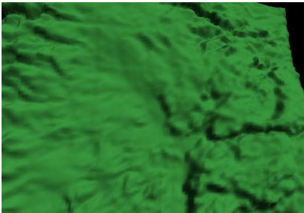
Figure (7) 3D view of the region with exaggeration.
