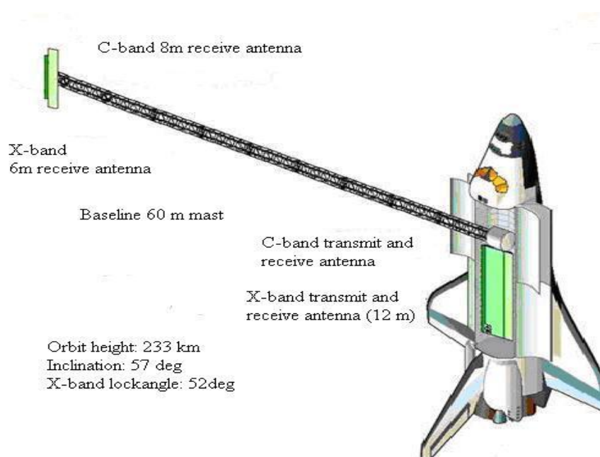
Figure (1) Shuttle Radar Topography Mission
