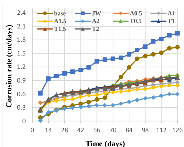
Figure 7. Corrosion rate over time (every 7 days) for a brine solution.
