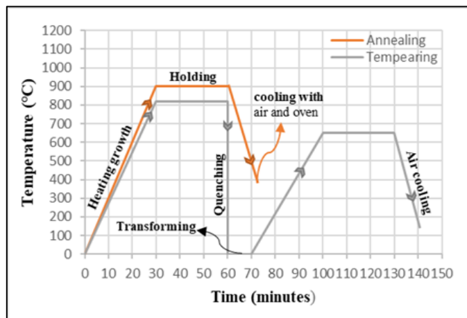
Figure 3. The heat treatment process.
