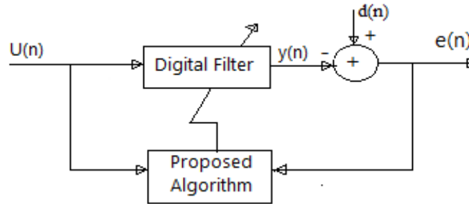
Fig. 2 Block diagram of an Adaptive Equalizer
