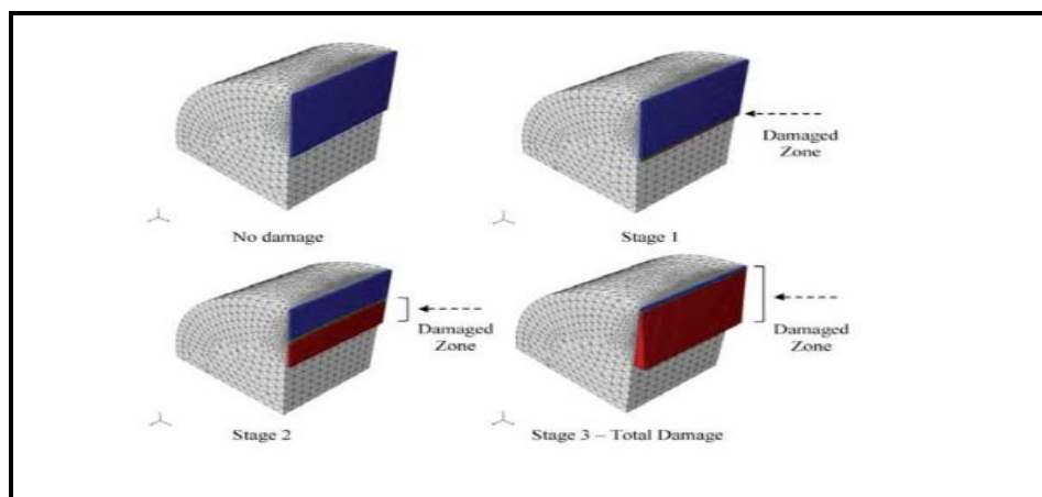
Fig.6: Damage evolution in the SCB test [114].
