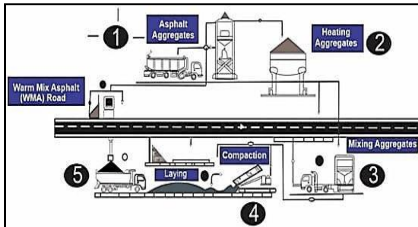
Fig. 3: Warm Mix Asphalt (WMA) process diagram [70]
