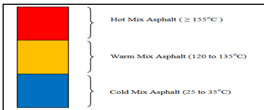
Fig.2: The usual range of temperatures for mixing asphalt mixes [61]
