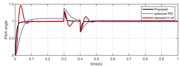
Fig. 8. Response pitch model for disturbance
