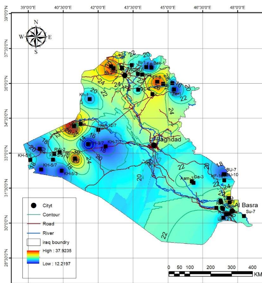
Fig. (1): Index map shows position of oil and water boreholes [11:12]
