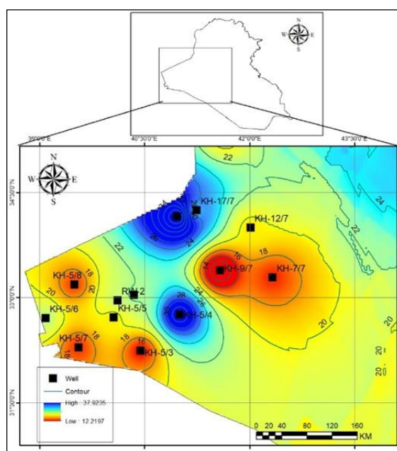
Fig. (4): Contour map showing geothermal gradient in Western Iraq
