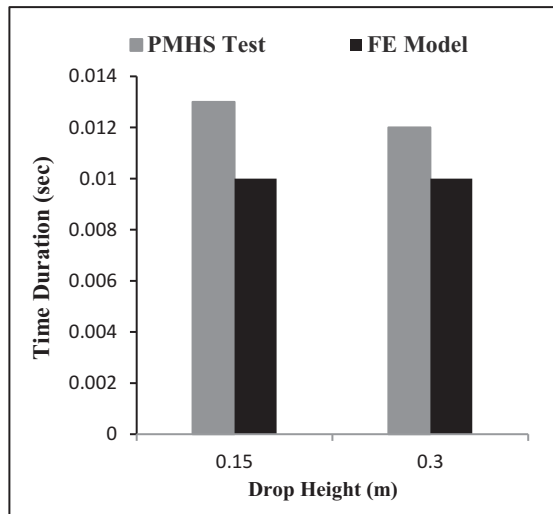
Fig. 7. The time at the point of head model impact is constructed on two different heights.
