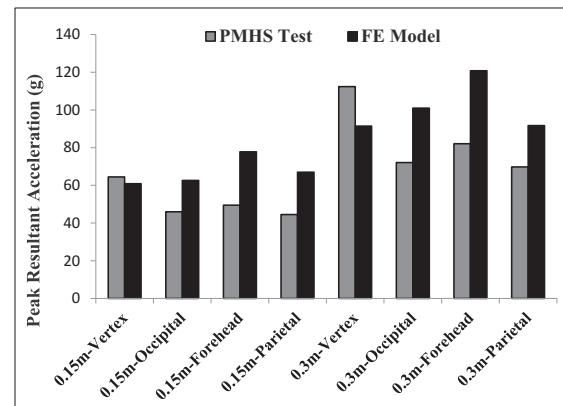
Fig. 6. The Peak resultant acceleration is established with different drop heights for head model impact tests.
