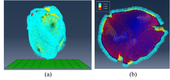
Fig. 3. The anisotropic properties of (a) the complete structure of the head model and (b) cranial bone.
