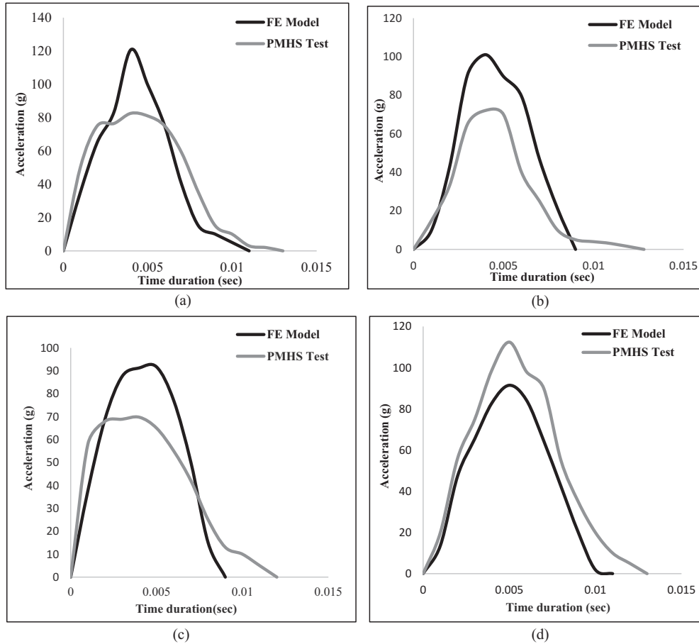
Fig. 5. The impact of the simulated model onto a rigid surface at the (a) forehead region (b) occiput region (c) parietal region (d) vertex region.
