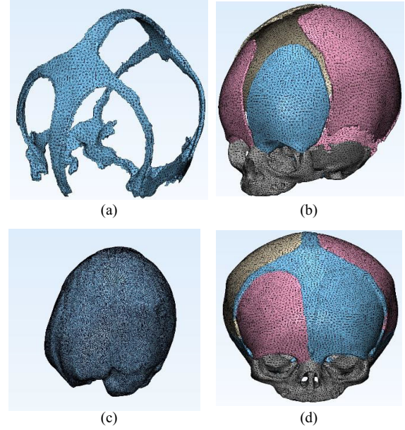
Fig. 2. The structures of the infant's head (a) sutures (b) cranial bones (c) brain (d) complete structure of the head.
