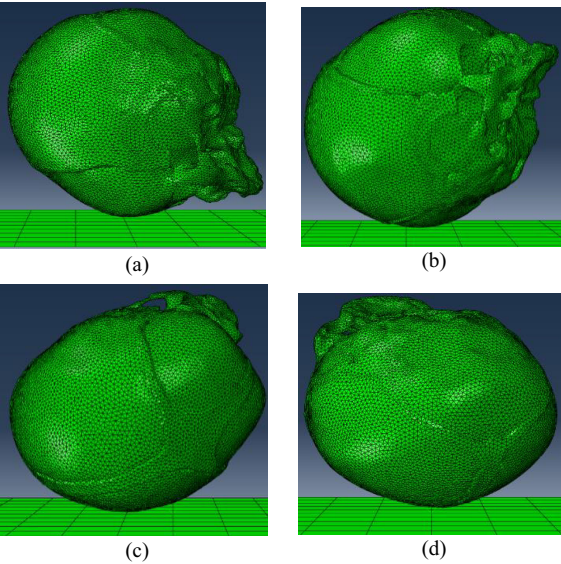
Fig. 4. The impact of the simulated head model onto a rigid surface at (a) Forehead region (b) Occiput region (c) Parietal region (d) Vertex region.
