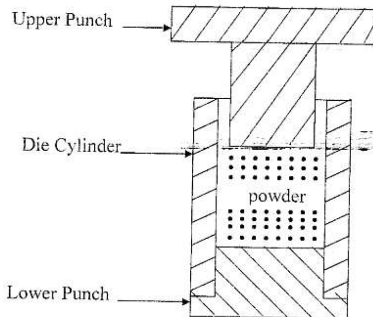
Fig. (2) Schematic diagram of the die assembly
