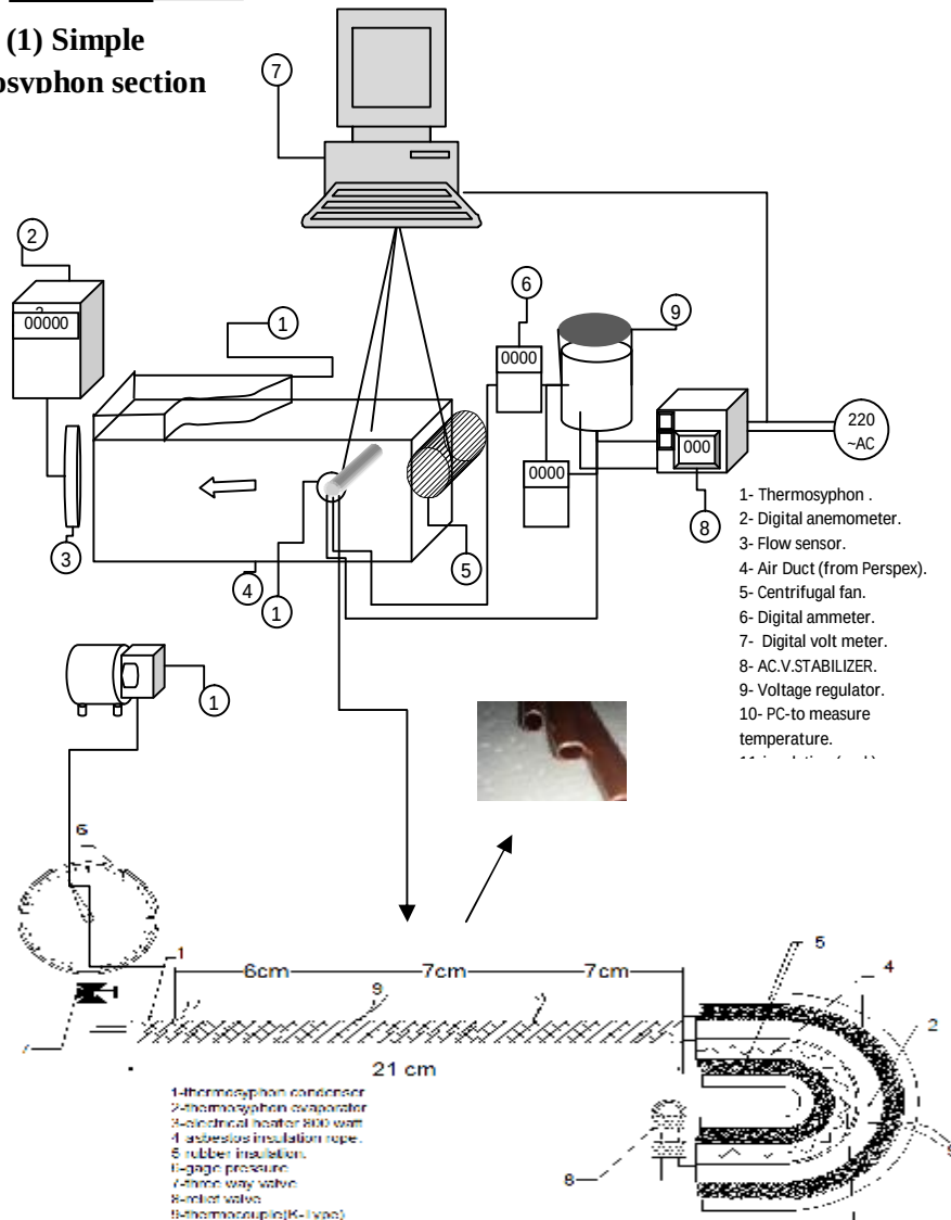
Figure (4) Schematic diagrams of experimental two phase
