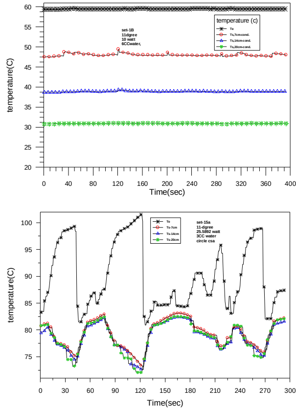
Figure (11) flow behavior (a) uniform flow and (b) alternative chaotic flow
