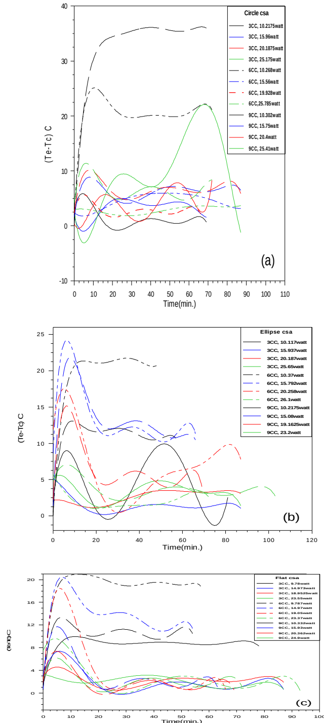
Figure9 (a-c) Temperature difference between evaporator and condenser for the three geometry (three RAP) , against time,(a-circ
