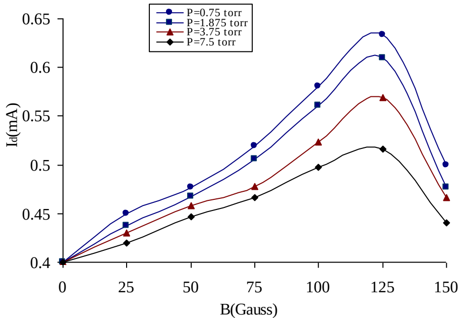
Fig. (7): Variation of discharge current with magnetic field for different pressures of \text{CO}_2 ( I_d=0.4\text{mA} )
