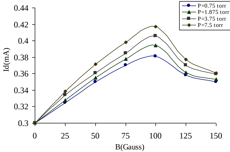
Fig. (6): Variation of discharge current with magnetic field for different pressures of \text{CO}_2 ( I_d=0.3\text{mA} )
