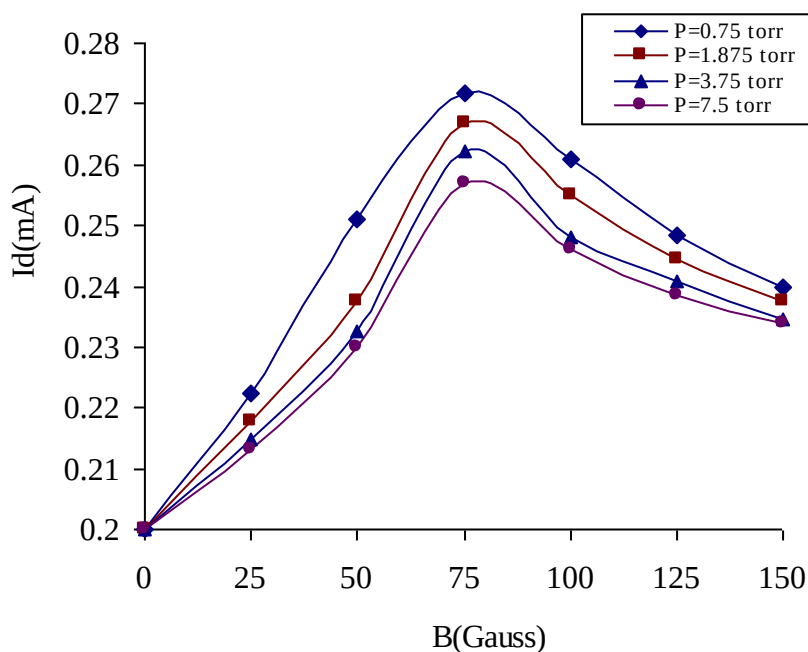
Fig. (5): Variation of discharge current with magnetic field for different pressures of CO_2 ( I_d=0.2 mA)
