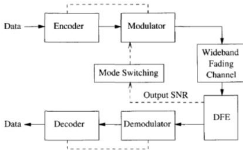
Figure (2). The burst-by-burst System without channel inter leaver.
