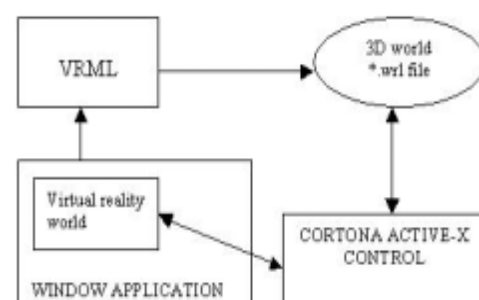
Figure 4 architecture of a virtual program [31]
