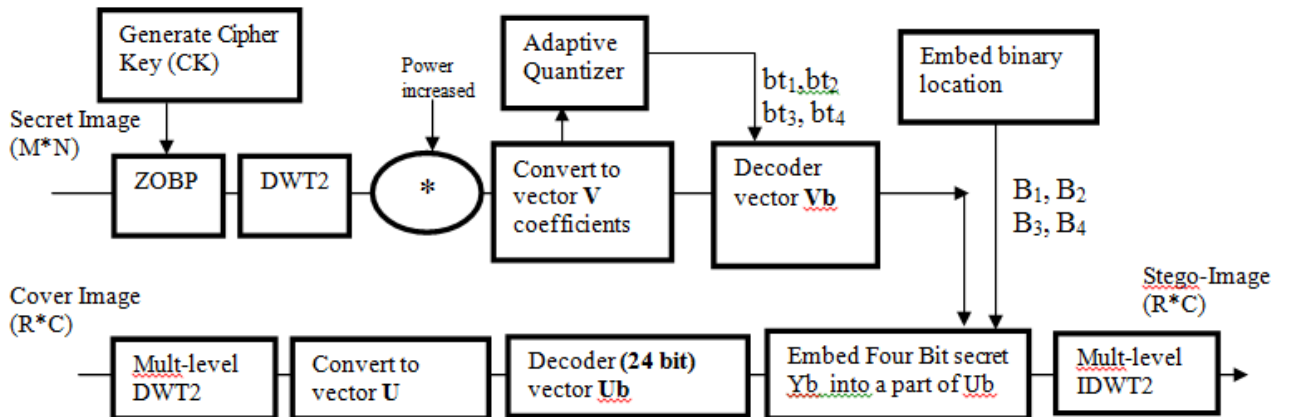
Fig. (3). Proposed Embedding System.
