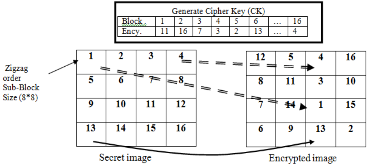
Fig. (2). Schematic of Encrypted System.
