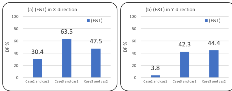
Figure7. The absolute values of DFs % of maximum displacement for (F&L) to cases 1-3 in (a)X- direction, (b) Y-direction.
