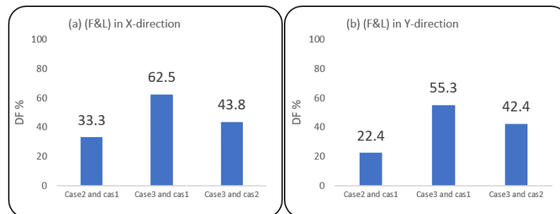
Figure18. The absolute values of maximum DFs (F&L) of M3 plastic hinge number for the cases 1-3 in (a)X-direction, (b) Y-direction.
