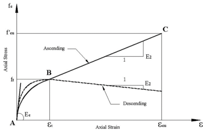
Fig. 3 Proposed model for FRP-confined concrete by (Youssef, 2007)
