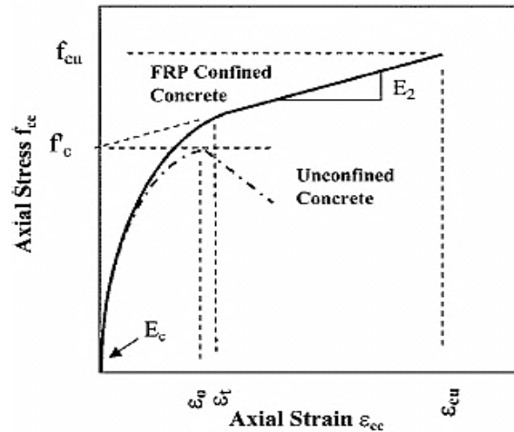
Fig. 1 Stress-strain model proposed by (Lam L. &, 2003)
