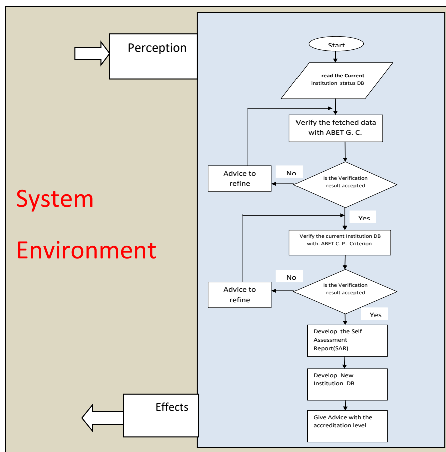
Figure( 3) Structure of the Assessment Agent
