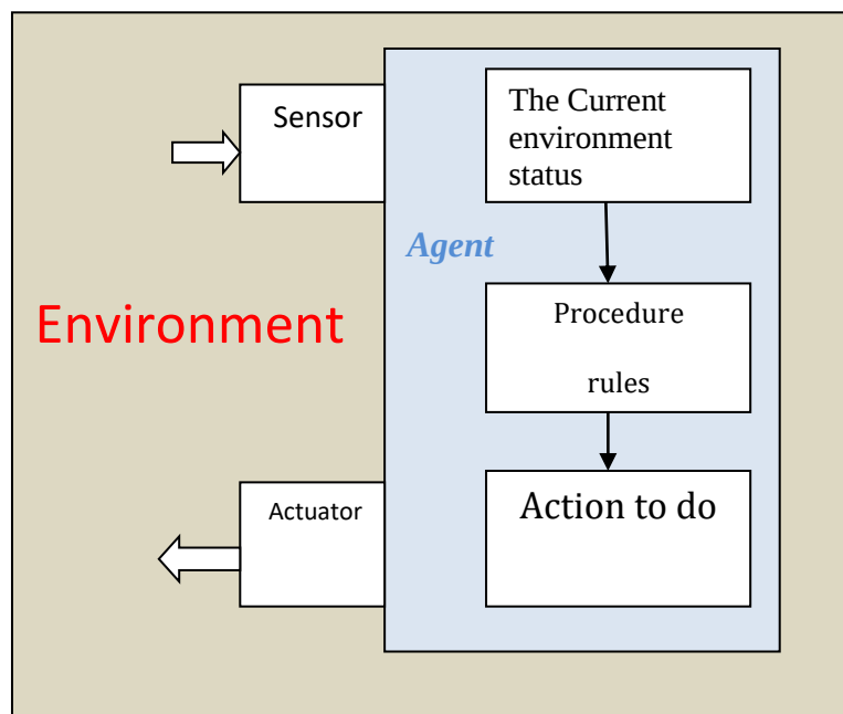
Figure(1) The principle structure of the software agent
