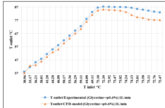
Fig. 17. The validation between Experimental (Glycerine+0.6%) and CFD-Model
