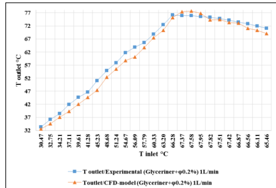
Fig. 15. The validation between Experimental (Glycerine+0.2%) and CFD-Model
