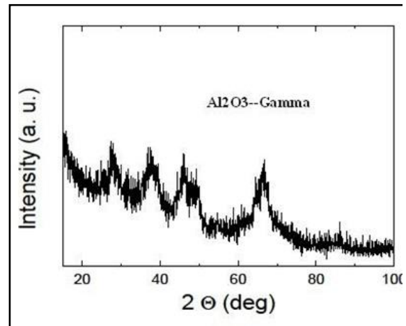
Fig. 5. X-Ray Al 2 O 3 -gamma Nanoparticles.
