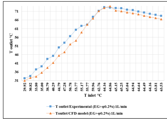
Fig. 20. The validation between Experimental(EG+0.2%) and CFD-Model
