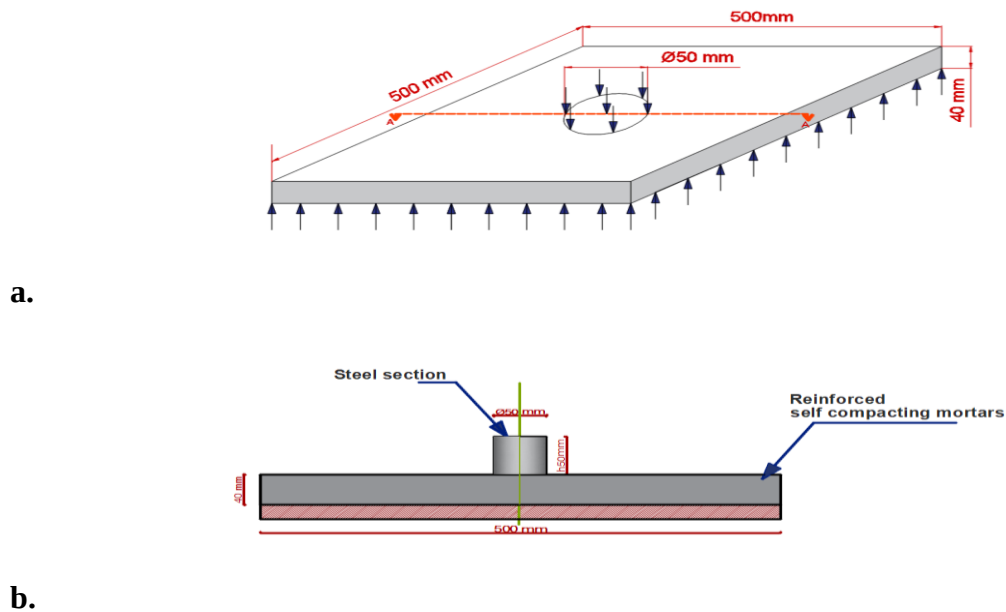
Fig. 1. Experimental setup: (a) Overall view; (b) Section (A-A).
