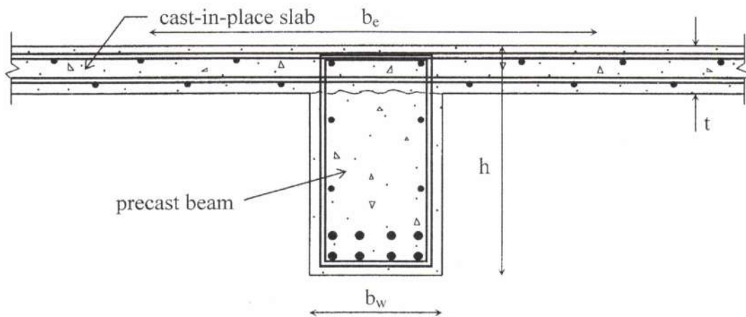
Fig. (1) Typical composite reinforced concrete beam.
