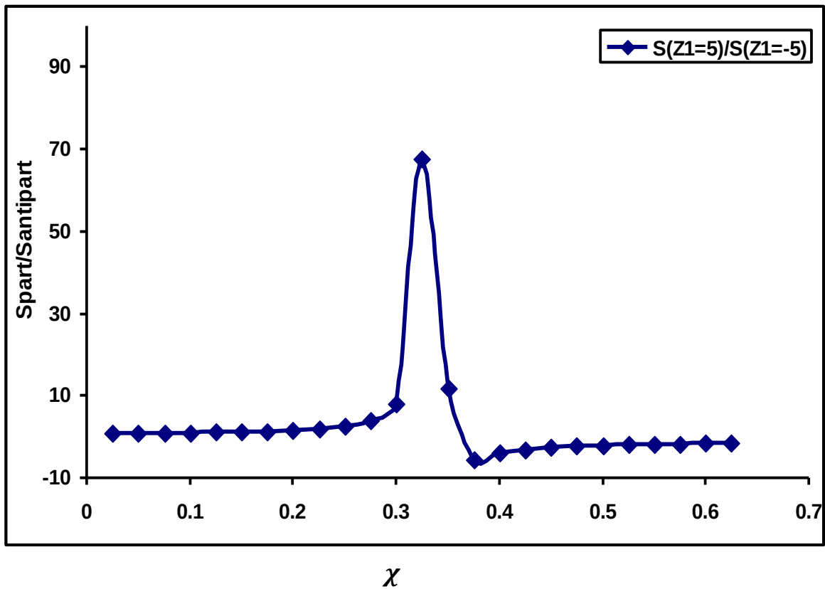
Fig.(5-b) Proportion of stopping power of particle ( Z_1 = 5 ) to antiparticle ( Z_1 = -5 ) with density parameter ( \chi )
