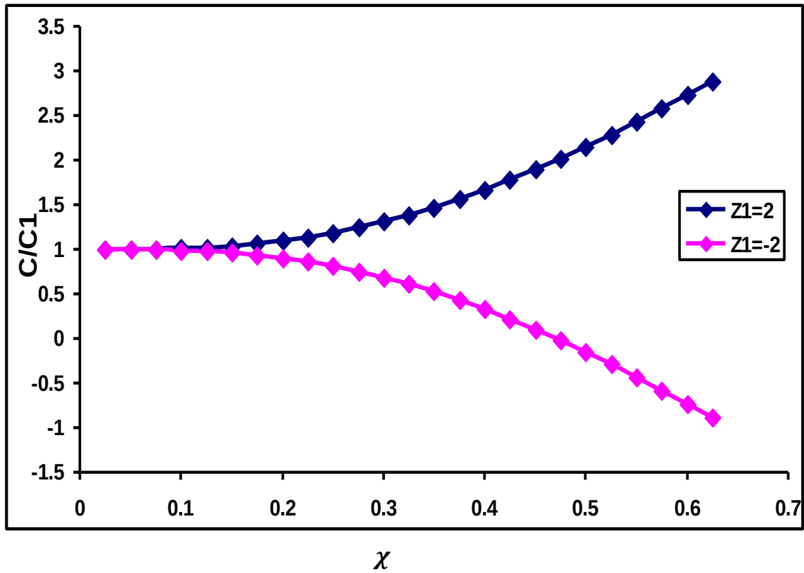
Fig.(6-a) Proportion of density function to the first Born approximation ( C/C_1 ) of particle ( Z_1 = 2 ) and antiparticle ( Z_1 = -2 ) with density parameter ( \chi )
