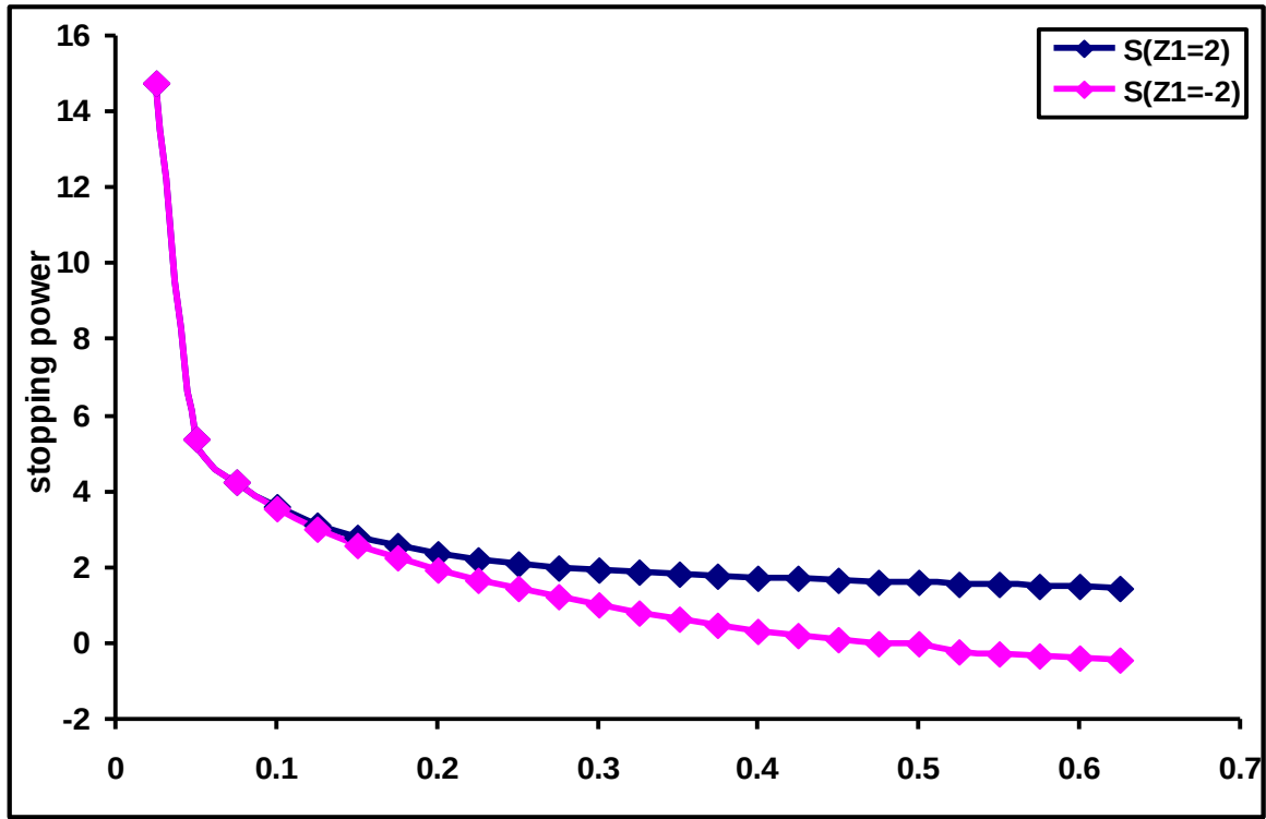
Fig.(4-a) Stopping power of particle ( Z_1 = 2 ) and antiparticle ( Z_1 = -2 ) with density parameter ( \chi )
