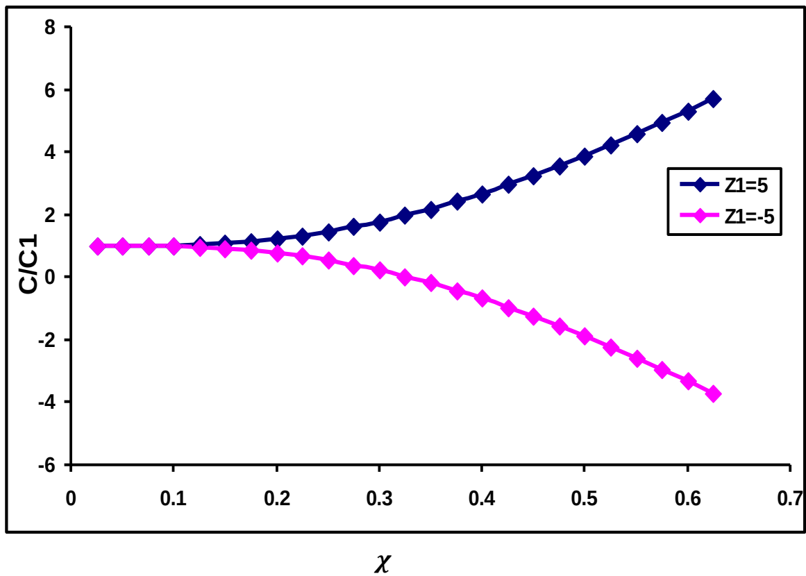
Fig.(6-b) Proportion of density function to the first Born approximation ( C/C_1 ) of particle ( Z_1 = 5 ) and antiparticle ( Z_1 = -5 ) with density parameter ( \chi )
