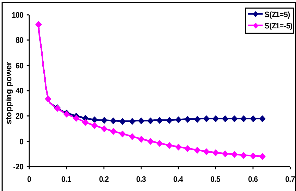
Fig.(4-b) Stopping power of particle ( Z_1 = 5 ) and antiparticle ( Z_1 = -5 ) with density parameter ( \chi )
