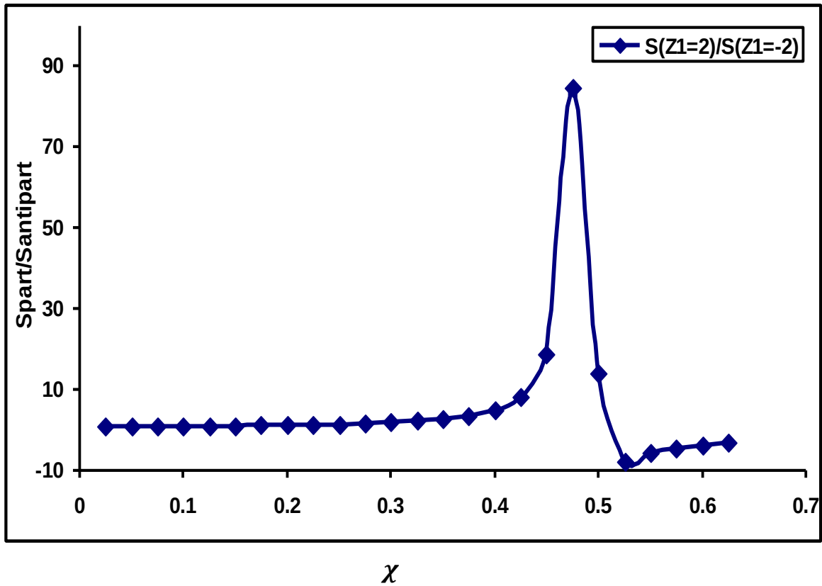
Fig.(5-a) Proportion of stopping power of particle ( Z_1 = 2 ) to antiparticle ( Z_1 = -2 ) with density parameter ( \chi )
