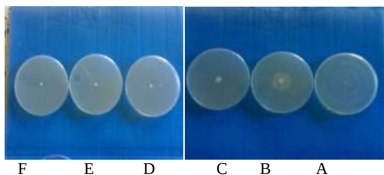
Figure (1) images of swarming on nutrient agar plates containing different concentrations of Alum (Aluminum potassium sulfate) at 37°C after 18 hrs inoculation. normal swarming phenomenon. B = 0.3 mg/ml began the inhibition of swarm. C=( 0.5 mg / ml) decrease the diameter of swarming . D= (0.6 mg / ml) Complete inhibition of swarming . E=( 0.7 mg/ ml) colony without swarming. F-( 0.8 mg/ ml) inhibition of growth.
