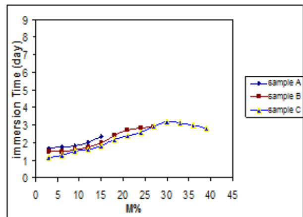
Figure (2) The Relative mass gain with the immersion time
