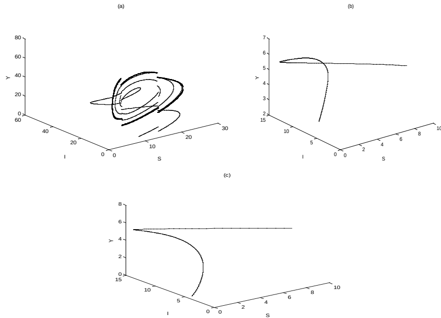
Figure (4): Phase plots of system (1). for data given in Eq.(10)(a) system (1) approaches to periodic attractor for \beta=0.05 , (b) system (2.1) approaches asymptotically to coexistence equilibrium point for \beta=0.5 , (c) system (1) approaches asymptotically to predator free equilibrium point on SI-plane for \beta=1 .
