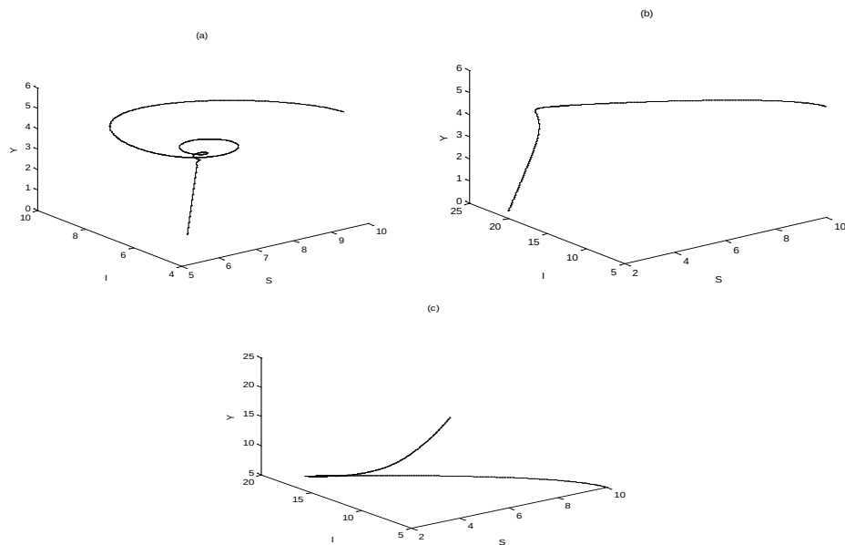
Figure (8): Phase plots of system (1) For the data given in Eq.(10)(a) system (1) approaches asymptotically to predator free equilibrium point on SI-plane for P_2 = 0.01 (b) system (1) approaches asymptotically to predator free equilibrium point on SI-axis
