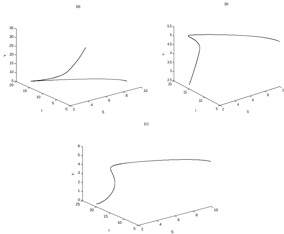
Figure(14): Phase plots of system (1) for the data given by Eq. (10) (a) system (1) approaches to asymptotically to coexistence equilibrium point for e_2=0.9 , ((b) system (1) approaches asymptotically to coexistence equilibrium point for e_2=0.3 , (c) approaches asymptotically to predator free equilibrium point on SI -Plane for e_2=0.01 .
