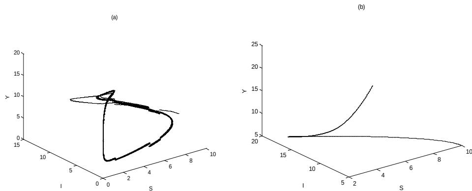
Figure (10): Phase plots of system (1) for the data given in Eq.(10) (a) system (1) approaches to periodic attractor for m=10 , (b) system (1) approaches asymptotically to coexistence equilibrium point for m=60
