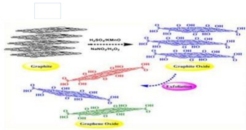
Figure (3): Mechanism of the prepared of graphene oxide (GO)
