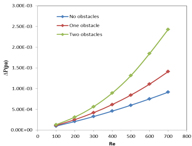
Fig. (8) Pressure drop with Reynolds number for different rectangular obstacle numbers.
