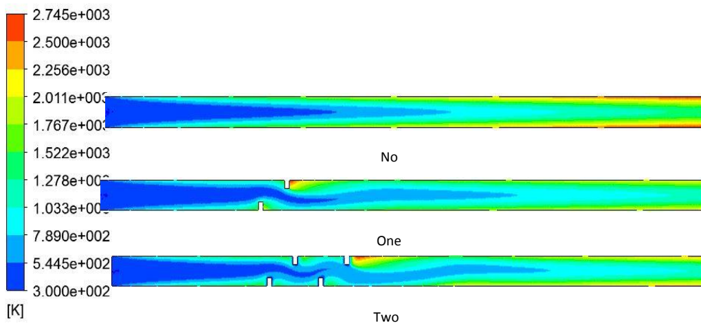
Fig. (6) Temperature distribution contours for rectangular obstacles at Re= 400
