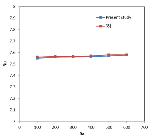
Fig.(3) Verification of Nusselt number of [8] with present study.
