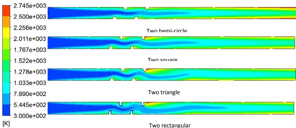
Fig. (11) Temperature distribution contours for different obstacle
