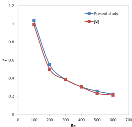
Fig. (2) Verification of friction factor of [8] with present study
