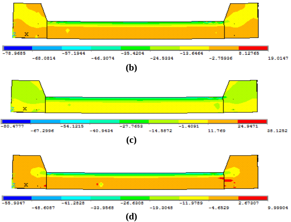
Fig. (21 ) Stress distribution in longitudinal x- direction of numerical columns at ultimate load level
