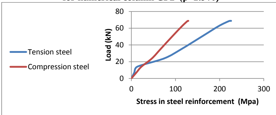
Fig. (9) Finite element stresses in steel bars at mid height versus load for numerical column CF3 ( \rho=3.2\% )
