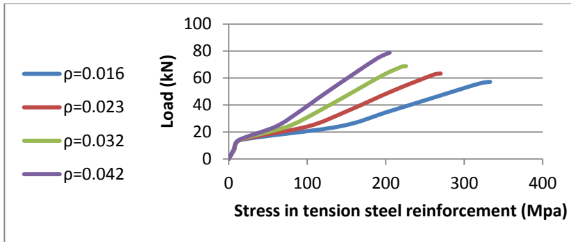
Fig. (5 ) Finite element tensile stresses in steel bars at mid height versus applied load for numerical columns (CF1,CF2, CF3 and CF4)
