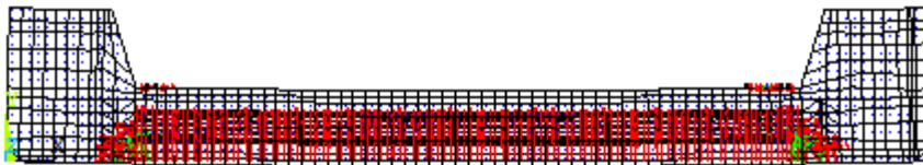
Fig. (22) Crack pattern of numerical column CF5 at ultimate load level.
