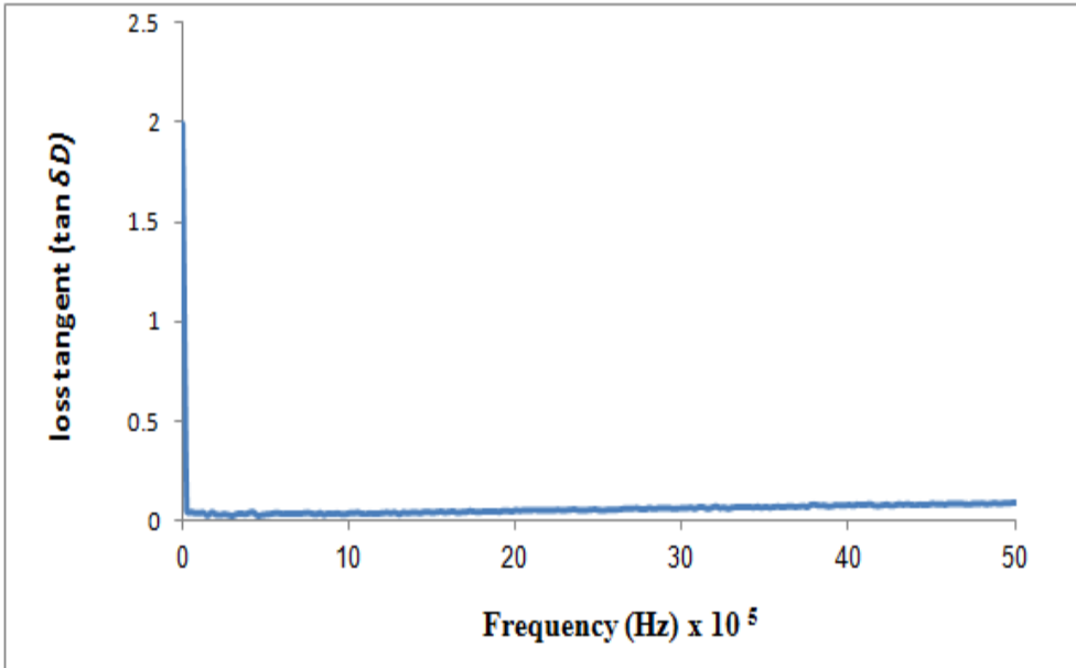
Figure (9) loss tangent ( \tan \delta_D ) versus of frequency for the porous silicon etching time was 10 min, and the current density was 15\text{mA/cm}^2 .
