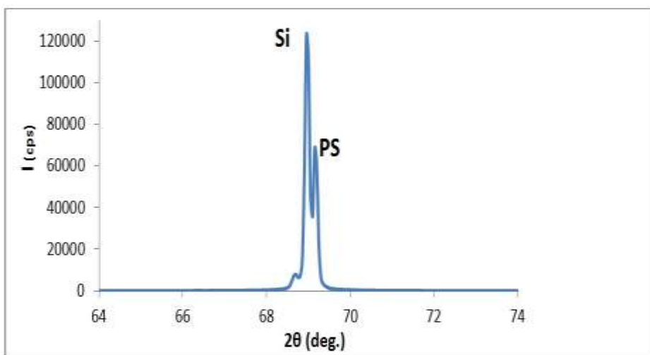
Figure (1) X-ray diffraction of porous silicon primed at anodizing time 10 min and current density 15 \text{ mA/cm}^2 .
