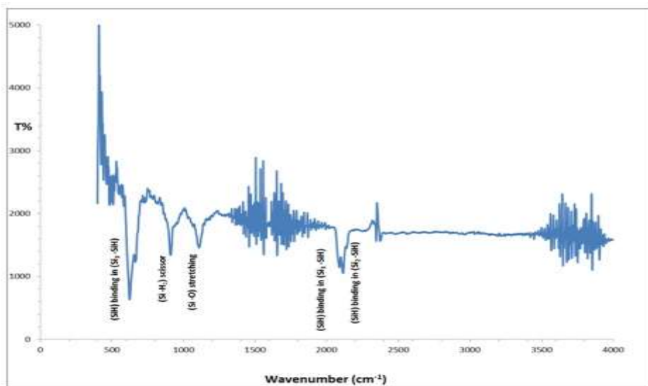
Figure (3) Fourier transform infrared transmittance spectrum of a PS layer 15 \text{mA/cm}^2 at etching time 10 min.
