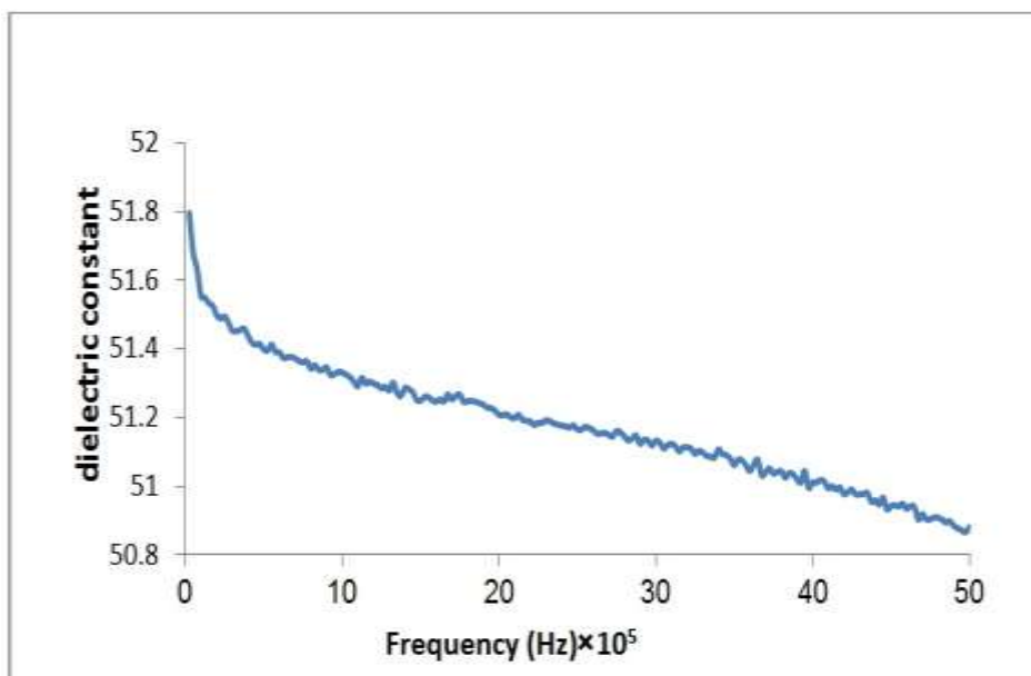
Figure (7) Dielectric permittivity as a function of frequency for the porous silicon etching time was 10 min, and the current density was 15mA/cm 2
