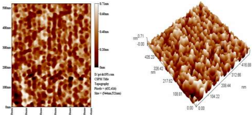
Figure (2) show 2D& 3D AFM images for meso-porous silicon sponge like At 15 mA/cm 2 and etching time 10 min.
