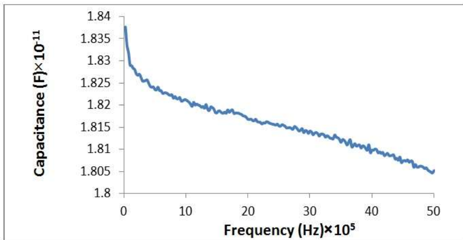
Figure (5) the capacitance as a functions of frequency for the porous silicon etching time was 10 min, and the current density was 15\text{mA}/\text{cm}^2
