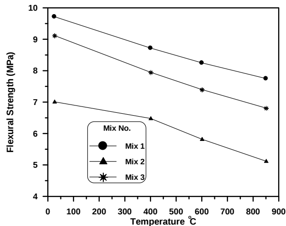
Figure (13): The effect of fire exposure on the flexural strength of high-strength concrete at age 90 days and 2.0 hours period of exposure.
