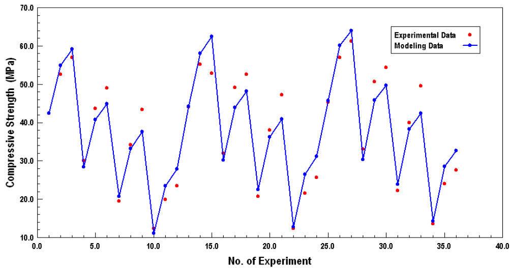
Figure 13: The difference between observed compressive strength and calculated compressive strength after burning in model (3).
