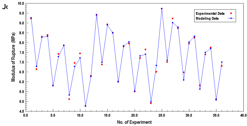
Figure 15: The difference between observed modulus of rupture and calculated modulus of rupture after burning in model (3).
