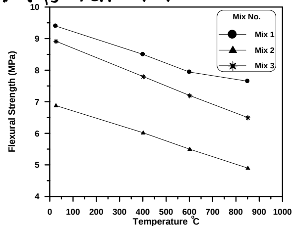
Figure (12): The effect of fire exposure on the flexural strength of high-strength concrete at age 60 days and 2.0 hours period of exposure.
