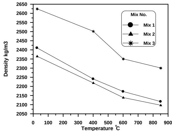
Figure (3): The effect of fire exposure on the density of high-strength concrete at age 90 days and 2.0 hours period of exposure.
