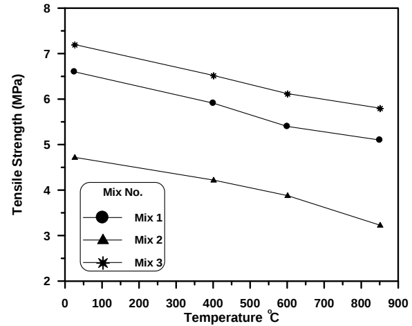
Figure (9): The effect of fire exposure on the tensile strength of high-strength concrete at age 60 days and 2.0 hours period of exposure.
