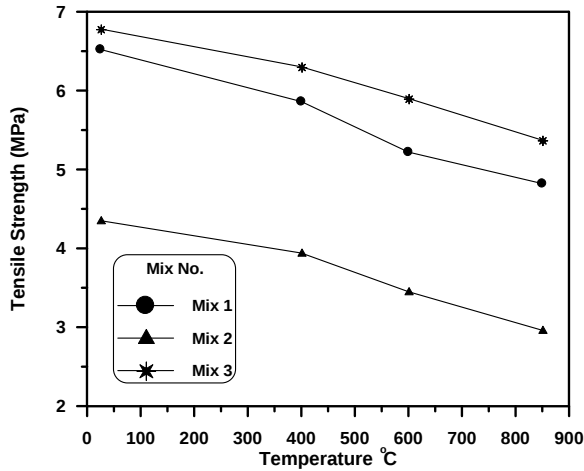
Figure (8): The effect of fire exposure on the tensile strength of high-strength concrete at age 30 days and 2.0 hours period of exposure.
