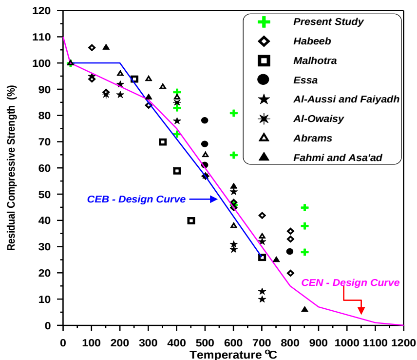
Figure (7): Comparison of residual compressive strength results and the recommended design curves of CEB and CEN.
