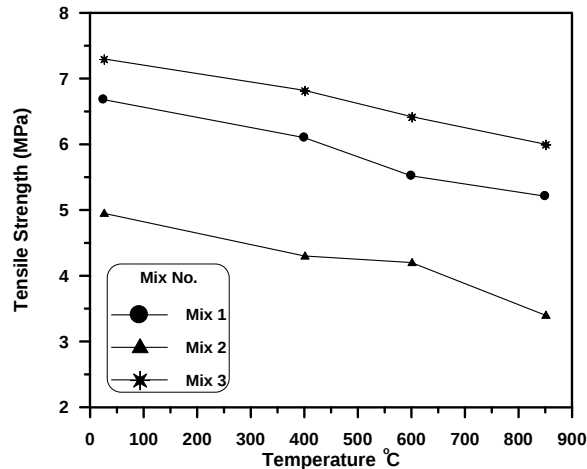
Figure (10): The effect of fire exposure on the tensile strength of high-strength concrete at age 90 days and 2.0 hours period of exposure.
