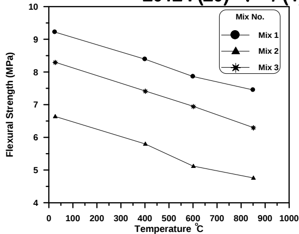
Figure (11): The effect of fire exposure on the flexural strength of high-strength concrete at age 30 days and 2.0 hours period of exposure.
