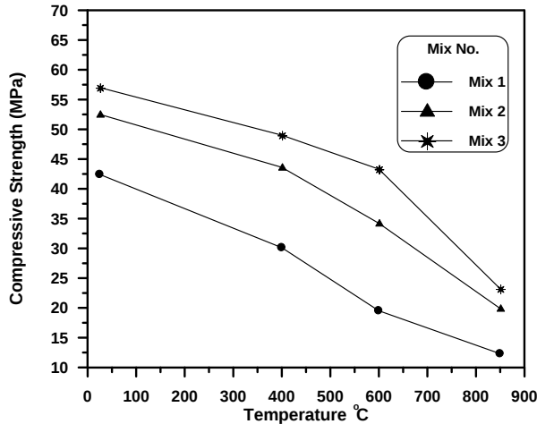
Figure (4): The effect of fire exposure on the compressive strength of high-strength concrete at age 30 days and 2.0 hours period of exposure.
