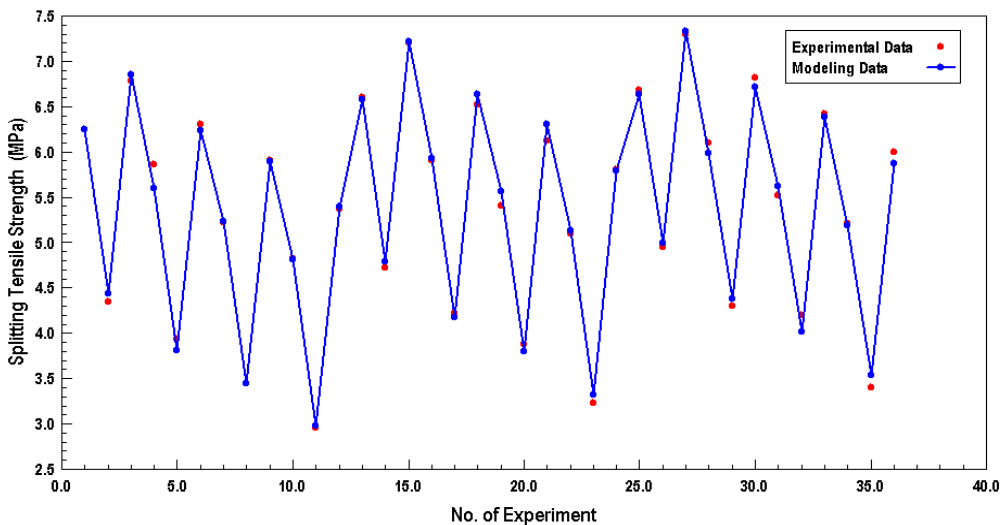
Figure 14: The difference between observed splitting tensile strength and calculated splitting tensile strength after burning in model (3).
