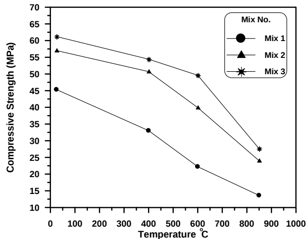
Figure (6): The effect of fire exposure on the compressive strength of high-strength concrete at age 90 days and 2.0 hours period of exposure.
