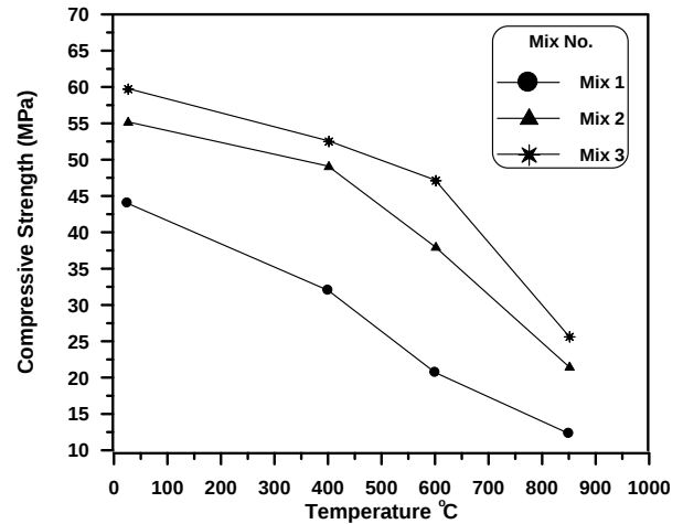
Figure (5): The effect of fire exposure on the compressive strength of high-strength concrete at age 60 days and 2.0 hours period of exposure.
