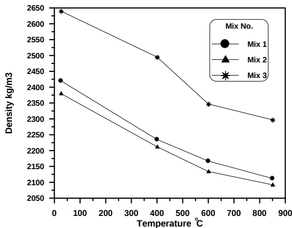
Figure (1): The effect of fire exposure on the density of high-strength concrete at age 30 days and 2.0 hours period of exposure.
