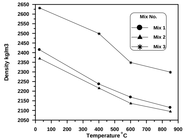
Figure (2): The effect of fire exposure on the density of high-strength concrete at age 60 days and 2.0 hours period of exposure.
