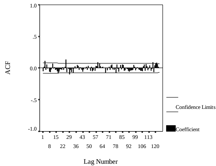
Fig.(5): Autocorrelogram of residual series parameter.
