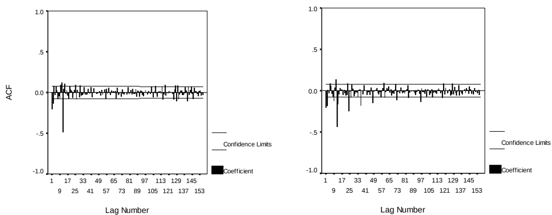
Figure 4: ACF and PACF of the series.
