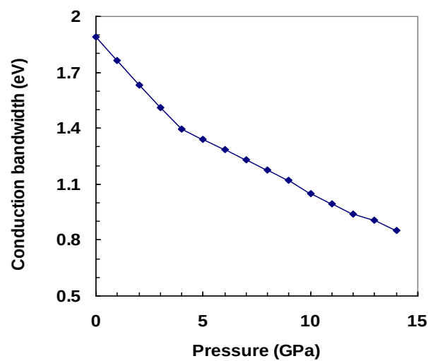
Figure 6. Predicted effect of pressure on the conduction bandwidth of ZnS.
