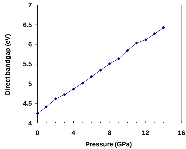
Figure 4. The effect of pressure on the bandgap of ZnS.
