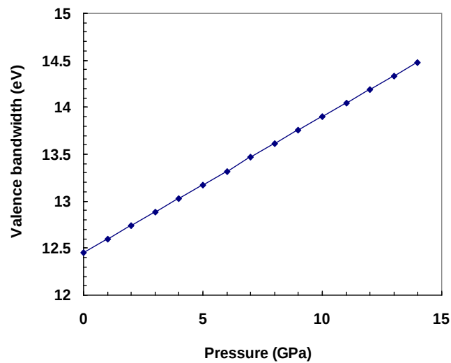
Figure 5. Pressure dependence of the valence bandwidth of ZnS.
