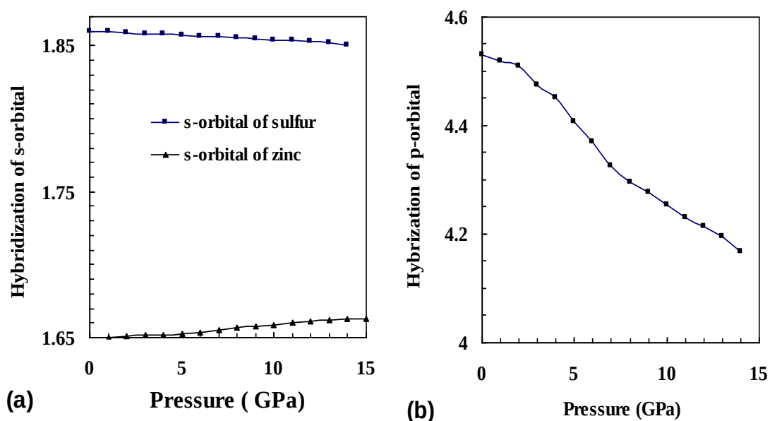
Figure 7. The effect of pressure on the hybridization of (a) s- state and (b) p- state.
