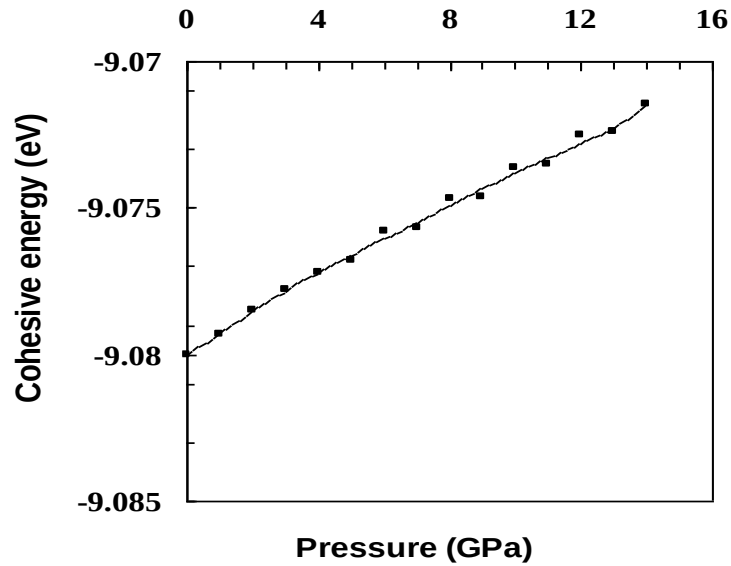
Figure 3. Cohesive energy versus pressure for ZnS.
