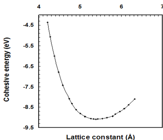
Figure 1. Cohesive energy as a function of lattice constant for ZnS.
