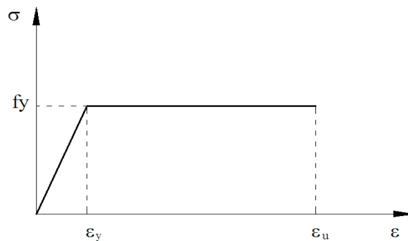
Fig.(3): Idealization of Stress-Strain Curve for Steel Beams.
