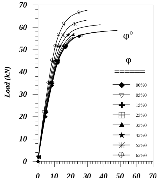
Figure (13): Load-Deflection
