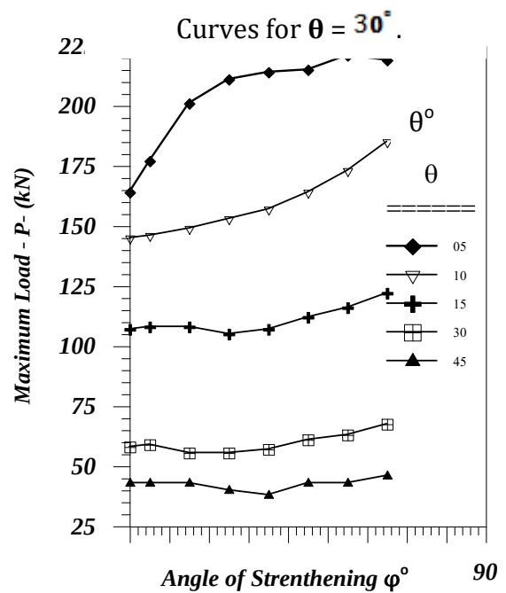
Figure (15): Ultimate Loads - Angles of Strengthening Curves.
