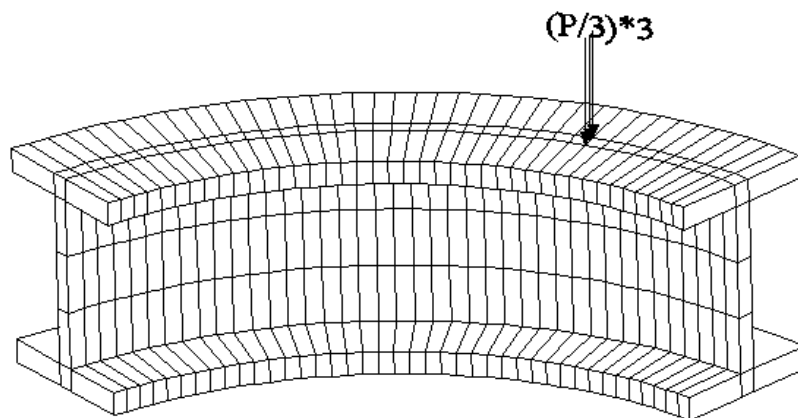
Fig.(6): Geometry, Properties and Loading Conditions of the Shanmugam Curved Beam(CB1).
