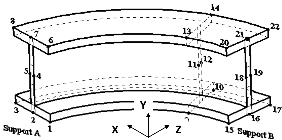
Fig.(5): Boundary Conditions in Finite Element Modeling.
