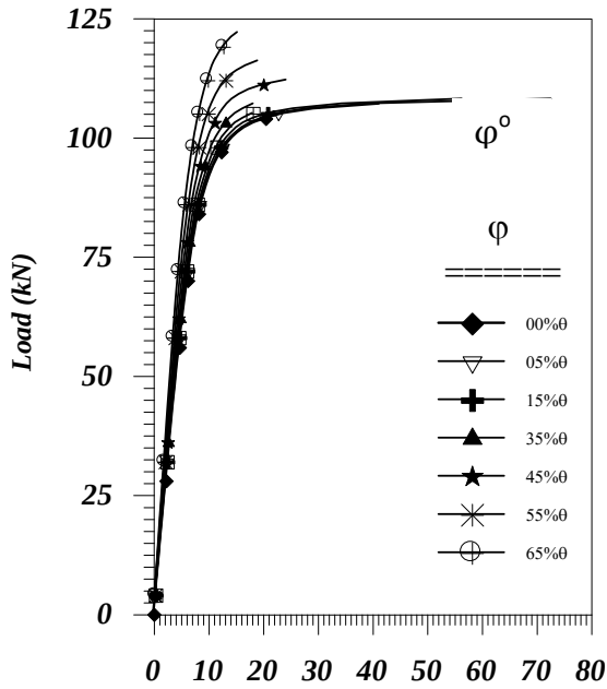
Figure (12): Load-Deflection
