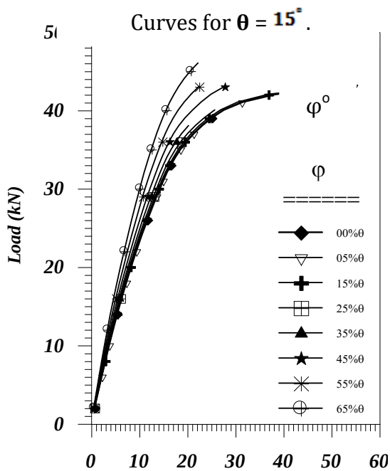
Figure (14): Load-Deflection
