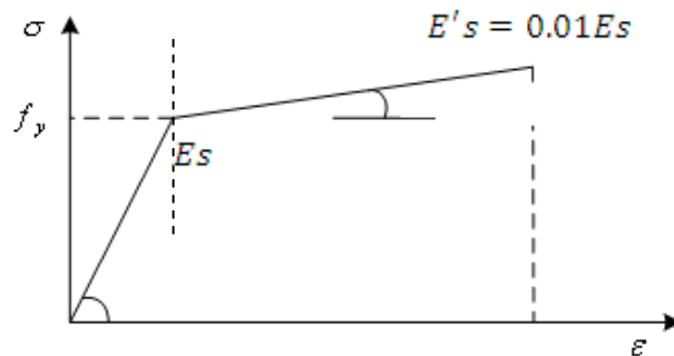
Figure 3: Elastio-plastic stress-strain relationships for steel(Xiong, and Zha, 2007)
