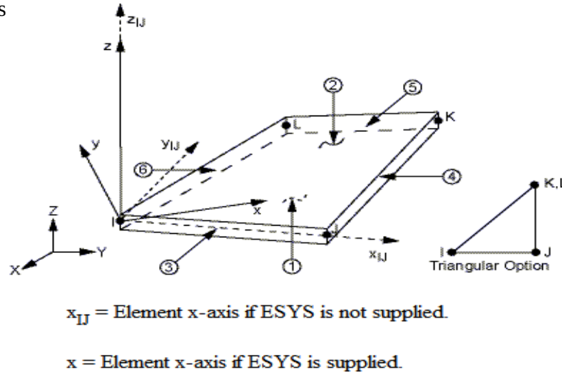
Figure 5: Element Geometry SHELL41(ANSYS, 2006).
