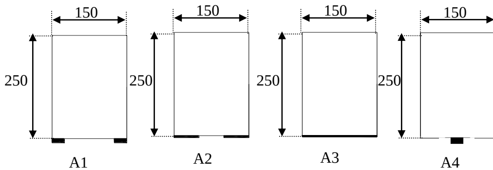
Figure 11: The locations of prestressed CFRP plate.
