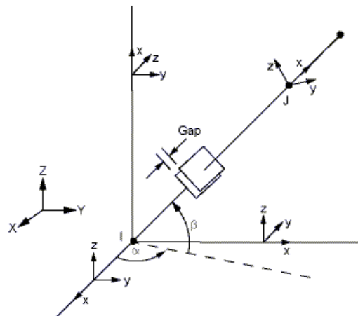
Figure 6: Element geometry CONTAC52(ANSYS, 2006).
