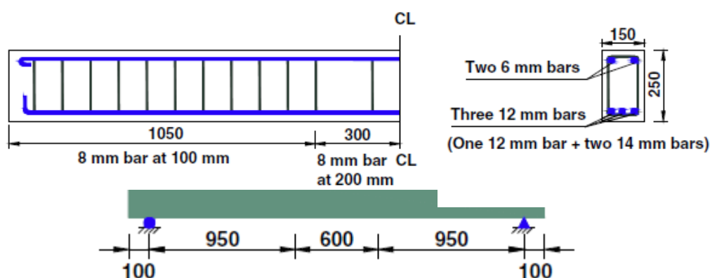
Figure 8: Reinforcement details of the concrete beam specimens (dimensions :mm) (Xue et.al., 2010)
