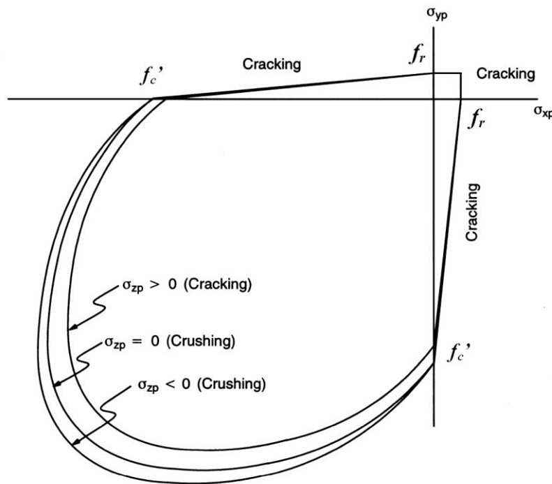
Figure 2: 3D-failure surface for concrete (ANSYS, 2006).
