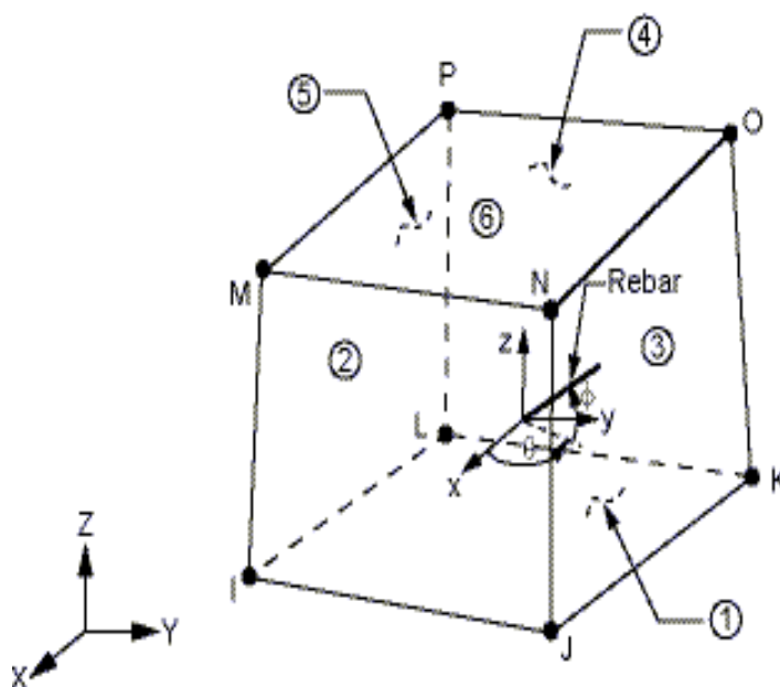
Figure 4: Element Geometry SOLID65 (ANSYS, 2006).
