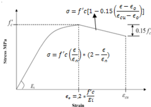
Figure 1 : Uniaxial stress-strain of concrete in compression(Hognestad, 1951).
