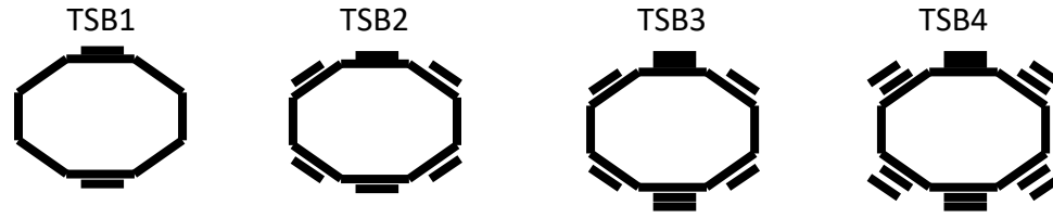
Fig. 2: The distribution Pattern of CFRP of the tested specimens
