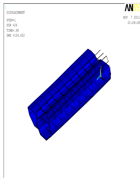
Fig. 14: Distribution of stresses intensity, Maximum displacement in Y direction and bulking of TSB2 beam by ANSYS-9.
