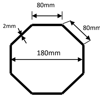
Fig 1: Section of specimen
