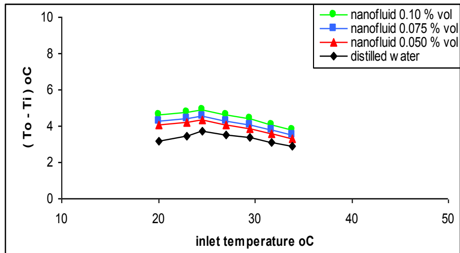
Figure 6: Temperature variation of inlet and outlet solar collector for ( \text{SiO}_2 + \text{DW} ) at various values of ( \phi\% ) and mass flow rate 20 L/h
