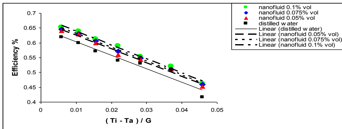
Figure 11: Collector efficiency at different ( \varphi %) and flow rate 10 L/h for nanofluid ( SiO_2+DW )
