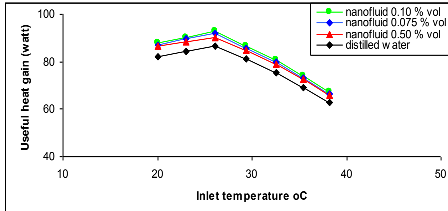
Figure 9: Useful heat gain variation of solar collector for ( \text{SiO}_2 + \text{DW} ) at different ( \varphi\% ) and mass flow rate 15 L/h
