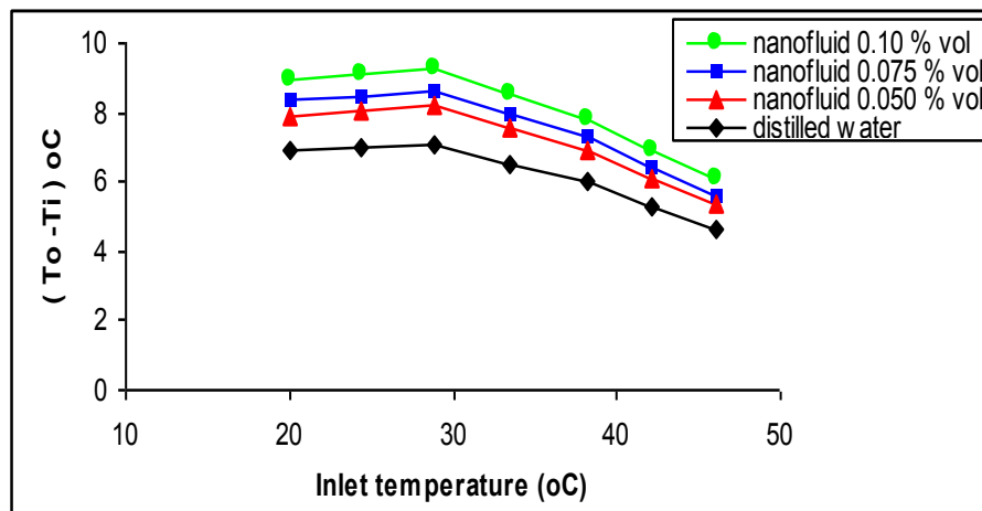
Figure 4: Temperature variation of inlet and outlet solar collector for (SiO 2 + DW) at various values of ( \phi %) and mass flow rate 10 L/h
