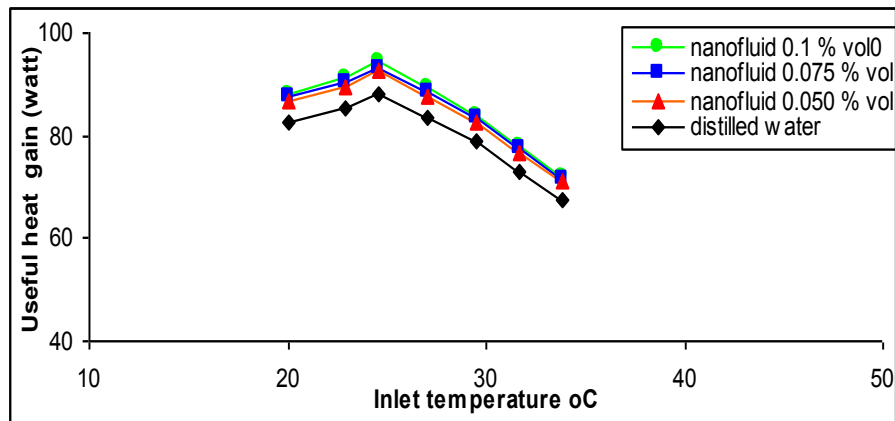
Figure 10: Useful heat gain variation of solar collector for ( \text{SiO}_2 + \text{DW} ) at different ( \varphi\% ) and mass flow rate 20 L/h
