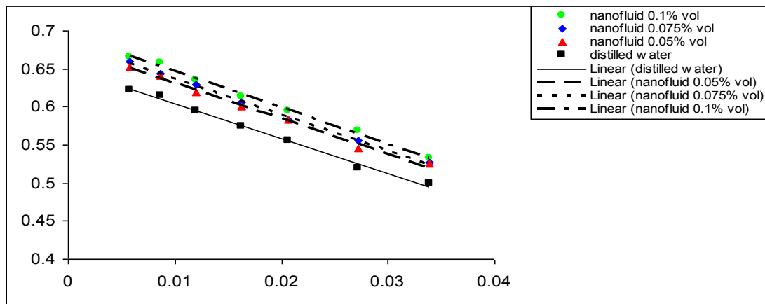
Figure 12: Collector efficiency at different ( \phi %) and mass flow rate 15 L/h for nanofluid ( \text{SiO}_2 +DW)
