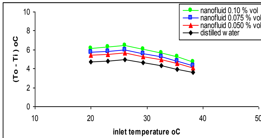
Figure 5: Temperature variation of inlet and outlet solar collector for (SiO 2 + DW) at various values of ( \phi %) and mass flow rate 15 L/h
