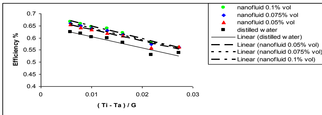
Figure 13: Collector efficiency at different ( \phi %) and mass flow rate 20 L/h for nanofluid ( \text{SiO}_2 +DW)
