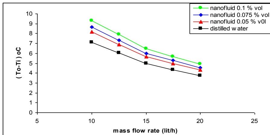
Figure 7: Difference comparison between maximum (inlet & outlet) temperature versus mass flow rate for ( \text{SiO}_2 + \text{DW} ) at different ( \phi\% )
