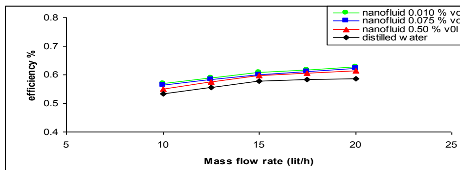
Figure 14: Variation of mass flow rate with efficiency at different ( \phi ) of nanofluid ( \text{SiO}_2 +DW)
