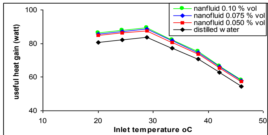
Figure 8: Useful heat gain variation of solar collector for ( \text{SiO}_2 + \text{DW} ) at different ( \phi\% ) and mass flow rate 10 L/h
