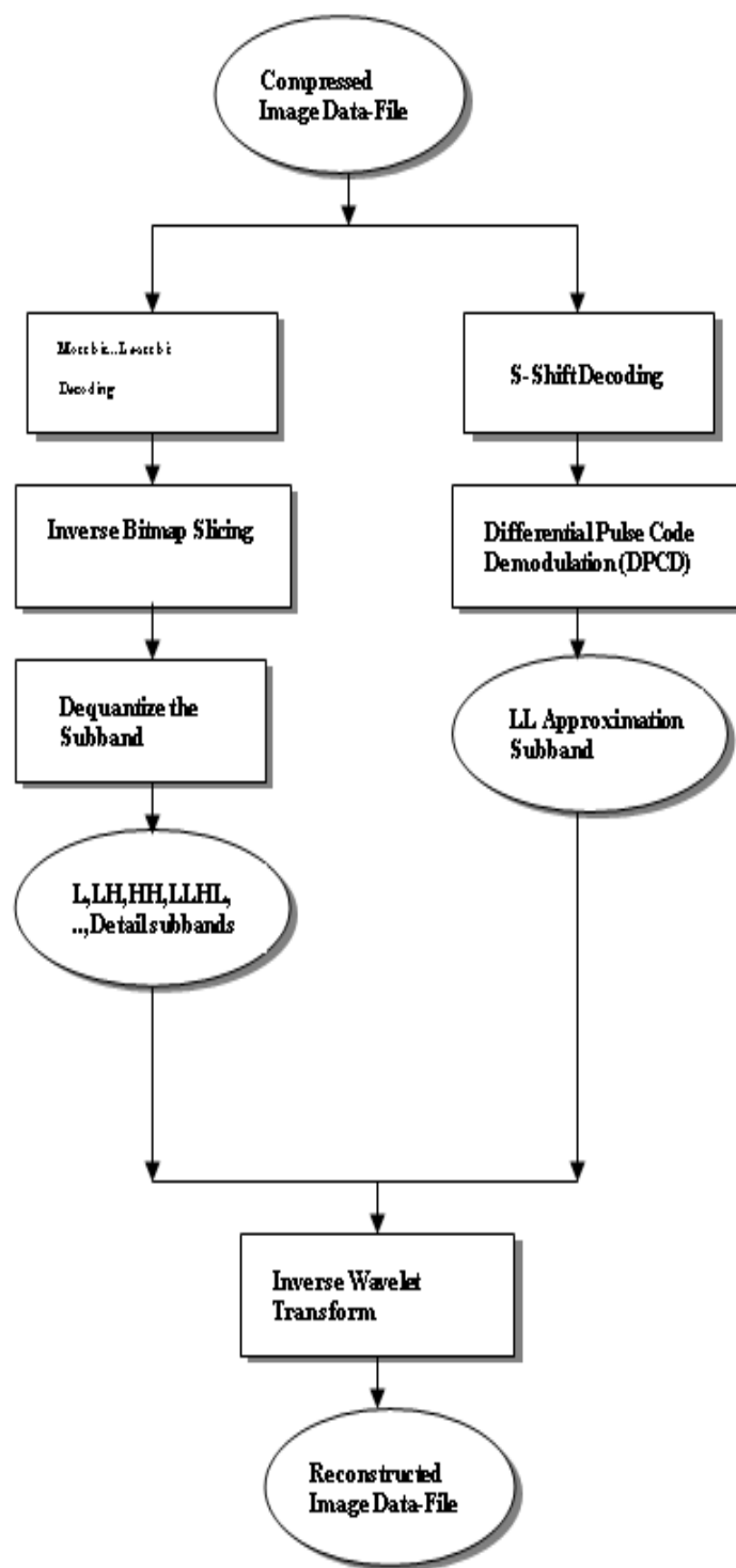
Figure (1).The suggested image compression system (A) and reconstruction system (B) based on based on wavelet transform
