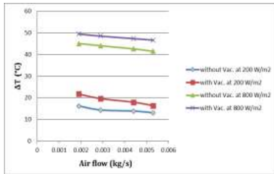
Figure 9: Experimental variance of temperature difference of air \Delta T (°C) with air flow at different values of irradiance with and without vacuum
