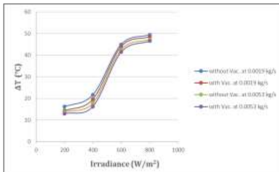
Figure 10: Variance of the temperature air difference with irradiance at various amounts of airflow with and without vacuum
