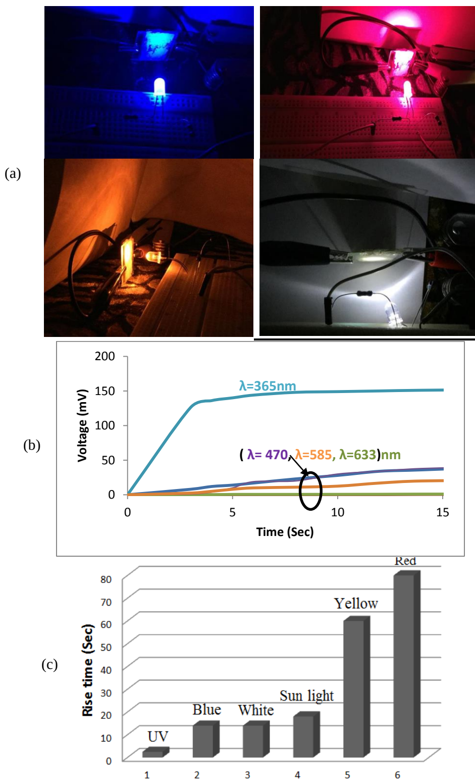
Figure (9): (a) Color testing setup. (b) Time response at various colors. Inset is the testing setup. (c) Rise time at various colors.
