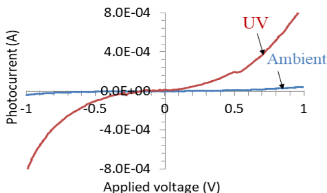
Figure ( 2): Electronic properties of the device in ambient and under UV illumination at \lambda=365 nm.
