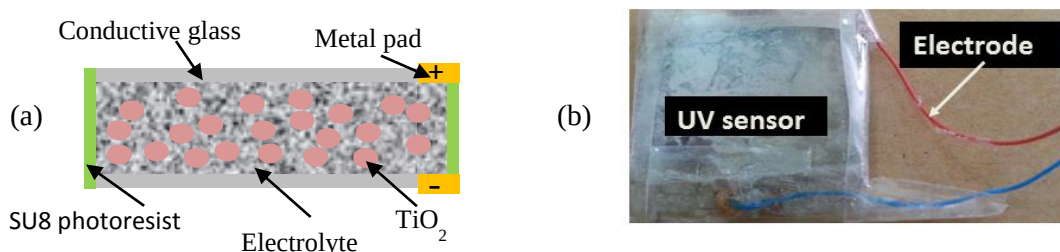
Figure (1): (a) Structure of the UV detector (b) Photo image of the detector after fabrication.
