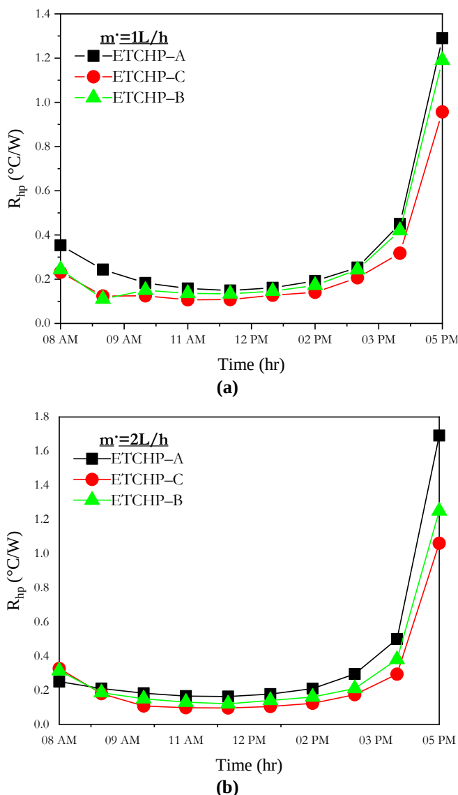
Fig. 7 Thermal resistance fluctuation for the HP throughout the charging time for (a) \dot{m} = 1 L/h (b) \dot{m} = 2 L/h.
