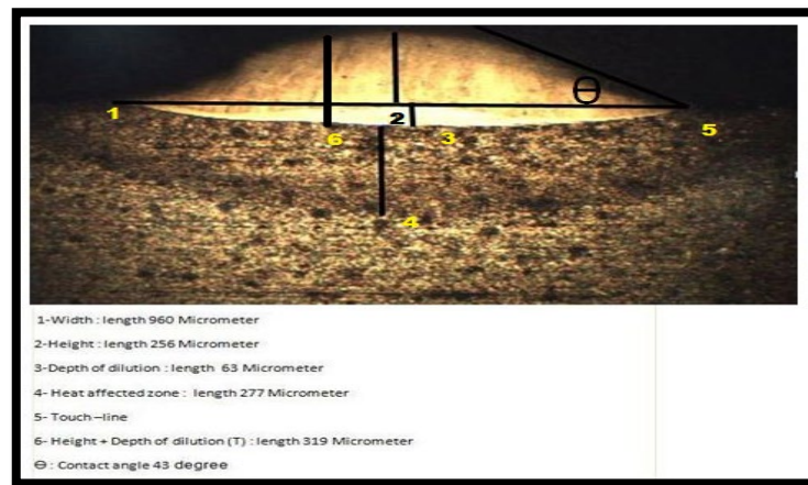
Figure 2: Six dimensions measured in electron microscopy.
