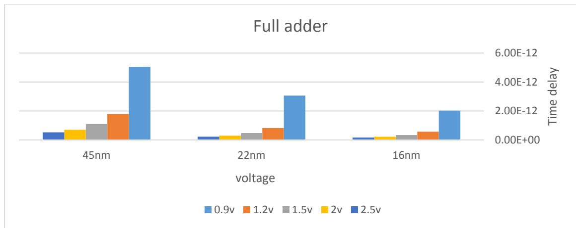
Figure 13: Time Delay 1-Bit FA Using the Power Model
