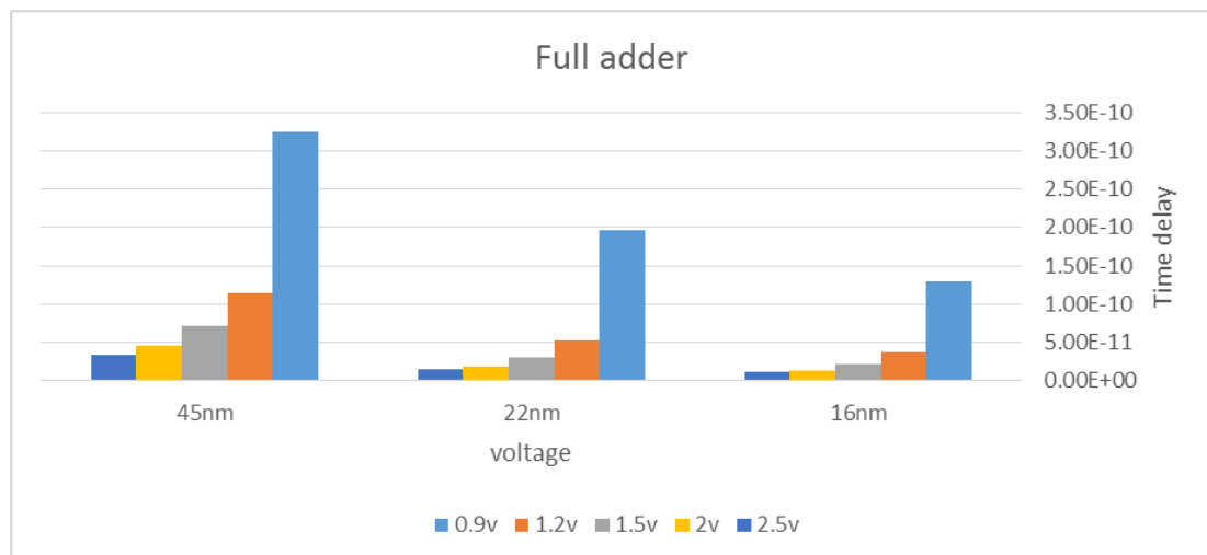
Figure 17: Time Delay 8-Bit FA Using the Power Model
