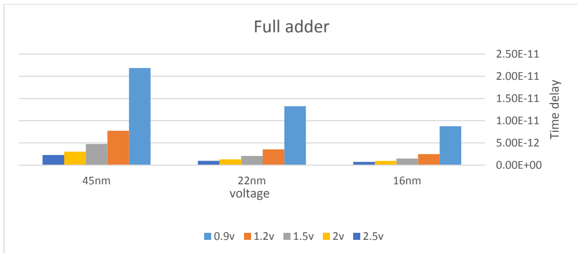
Figure 15: Time Delay of 4-Bit FA Using the Power Model
