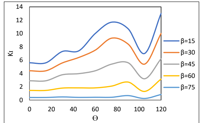
(a) K_I
