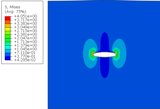
Fig. 5 stress distribution fringes.
