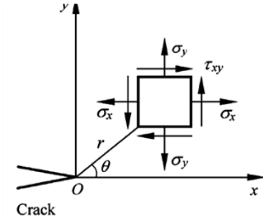
Fig. 1 Stress element at the crack tip.
